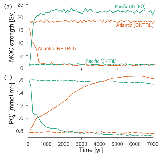
Figure 1. Time series (100-year means) of meridional overturning circulation for the Atlantic (orange) and Pacific (turquoise) at 30^\circ\ N (a); a water mass tracer ( PO_4^* ) at two locations in the northern Atlantic (mean of 28\text{--}38^\circ\ N , 60\text{--}70^\circ\ W ) and northern Pacific (mean of 28\text{--}38^\circ\ N , 150\text{--}160^\circ\ W ) (b). RETRO is shown by the solid lines and CNTRL by the dashed lines in both panels. PO_4^* ( PO_4 + O_2/172 - 1.5 ) combines concentrations of phosphate and oxygen in such a way that, to first order, biological impacts are eliminated and thus can be used as a (quasi-)conservative property, which in the prograde world is used to track the contributions of North Atlantic deep water (NADW) and Antarctic bottom water (AABW) to the ventilation of the deep Pacific and Indian Ocean (Rae and Broecker, 2018).
