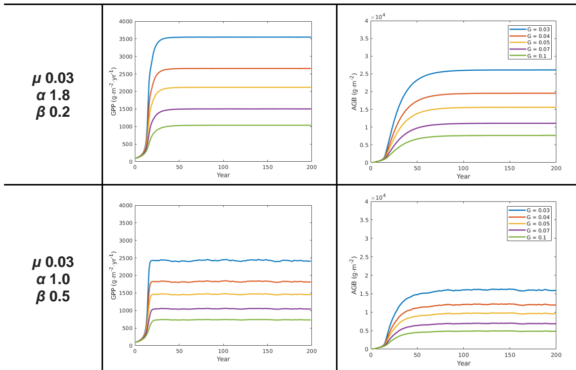
Figure S2. AGB ( gC \cdot m^{-2} ) and GPP ( gC \cdot m^{-2} \cdot yr^{-1} ) evolution against age (year) for different disturbance regimes
