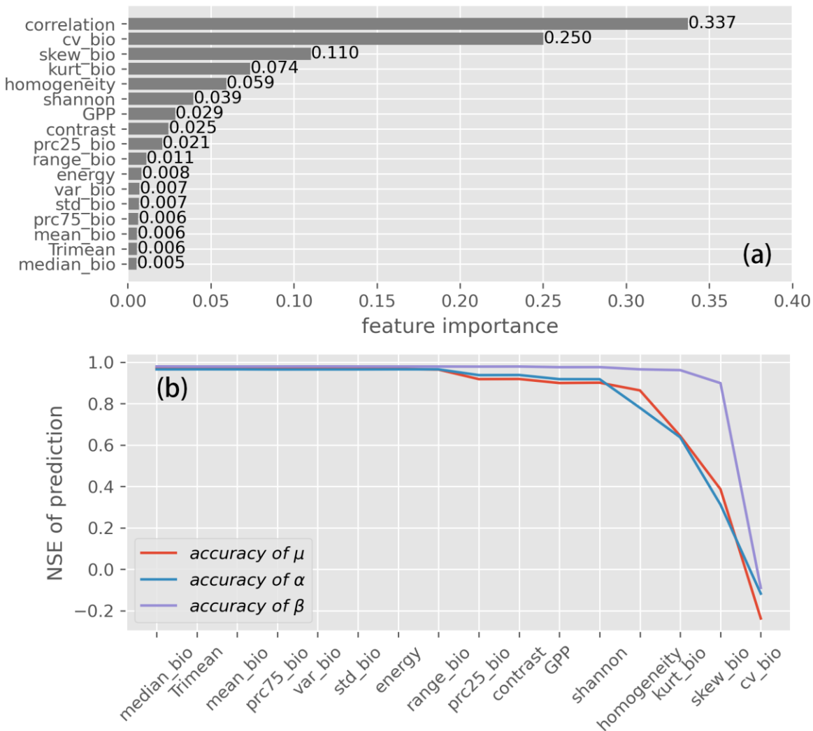
500 Figure 7. (a) shows the feature importance of multi-output disturbance regime prediction, the value for 505 each feature represents the magnitude of the accuracy decrease when removing its variability from the prediction of all three disturbance regime parameters; and (b) shows the prediction accuracy change in ascending importance for each disturbance regime parameter, x-axis refers to the feature(s) excluded from the prediction process (cumulatively from left to right). Accuracy is measured as the NSE between the full model estimates and the model outputs from the different factorial experiments for the entire three disturbance regime metrics ( \mu , \alpha , \beta ).
