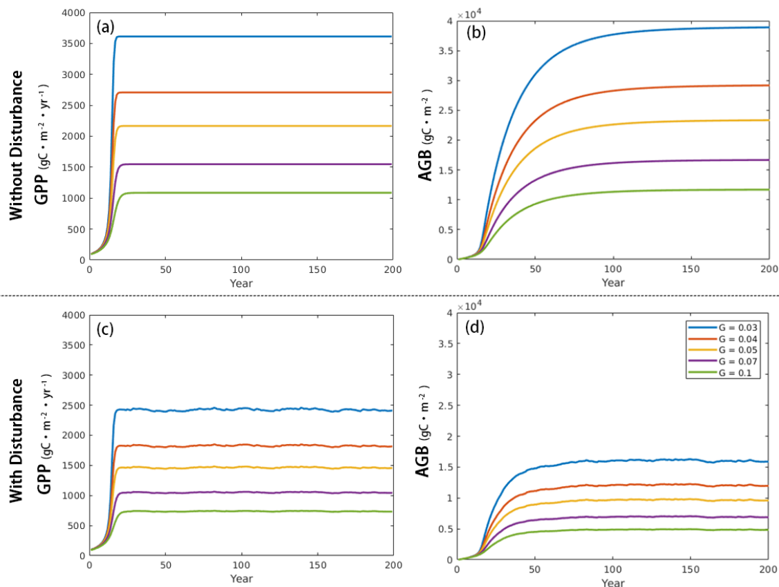
440 Figure 4. AGB and GPP evolution with varied Parameter G, (a) and (b) refer to the scenario without any disturbance events, (c) and (d) provide the impact of disturbance regime with \mu -0.03, \alpha -1.0, and \beta -0.2.
