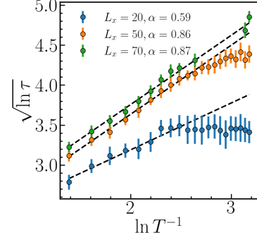
FIG. 9. Scaling of the prethermal lifetime of edge current for different system sizes L_x = 20, 50, 70 . We use parameters \delta J = 1J_0 , \delta h = 5J_0 , h_{max} = 6J_0 and T^{-1} in the unit of J_0 .
