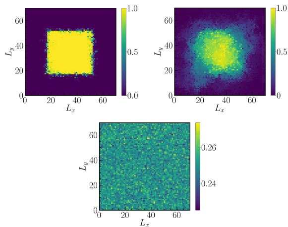
FIG. 5. Evolution of the particle density under Thue-Morse driving for a single random disorder realization for 1/T = 20J_0 . The times shown in the three panels correspond to 2^{15}T , 2^{25}T , 2^{35}T . The parameters are \delta J = 1J_0 , h_{\max} = 20J_0 , \delta h = 7J_0 .
