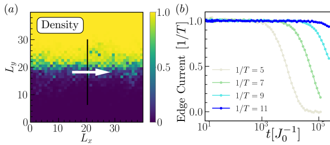
FIG. 4. (a) Particle density for a single 3–RMD realization at time t \approx 400J_0^{-1} for 1/T = 9 . (b) Edge current averaged over a single block at the boundary between filled and empty sites with 3–RMD for different driving frequencies. We use parameters \delta J = 1J_0 , h_{\max} = 10J_0 , \delta h = 7J_0 . T^{-1} is in units of J_0 .
