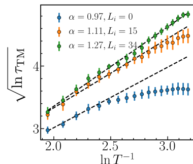
FIG. 7. Scaling of the delocalization time versus driving rates for different L_i . We use parameters L_x = L_y = 70 , \delta J = 1J_0 , \delta h = 7J_0 , h_{\max} = 6J_0 . T^{-1} is in the unit of J_0 .
