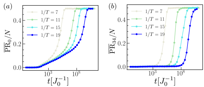
FIG. 6. Dynamics of \overline{\text{PR}}_{L_i}/N for initial states prepared at L_i sites away from the boundary of the cylinder of size 70 \times 70 . L_i = 0 and 34 in panel (a) and (b), respectively. We use parameters L_x = L_y = 70 , \delta J = 1J_0 , \delta h = 7J_0 , h_{\max} = 6J_0 . T^{-1} is in the unit of J_0 .
