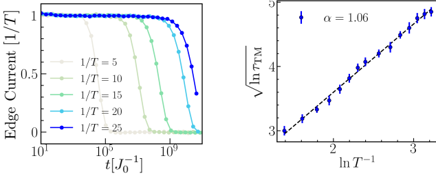
FIG. 8. Dynamics of the edge current and its lifetime scaling for L_x = L_y = 70 . We use parameters \delta J = 1J_0 , \delta h = 7J_0 , h_{max} = 6J_0 and T^{-1} in the unit of J_0 .
