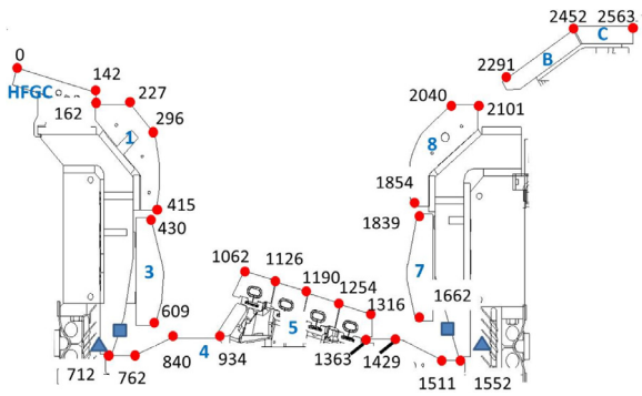
Fig. 1. Cross section of JET-ILW divertor showing tile numbering and the s -coordinate; distance around the divertor surface in millimetres. Tile 1 apron is in the region s = 162\text{--}227 mm. Tile 5 is also referred to as the bulk tungsten tile. \blacktriangle shows the location of louvre clips. \blacksquare shows the location of mirrors.
