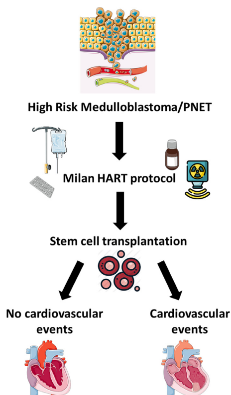
Figure 1. Study design
