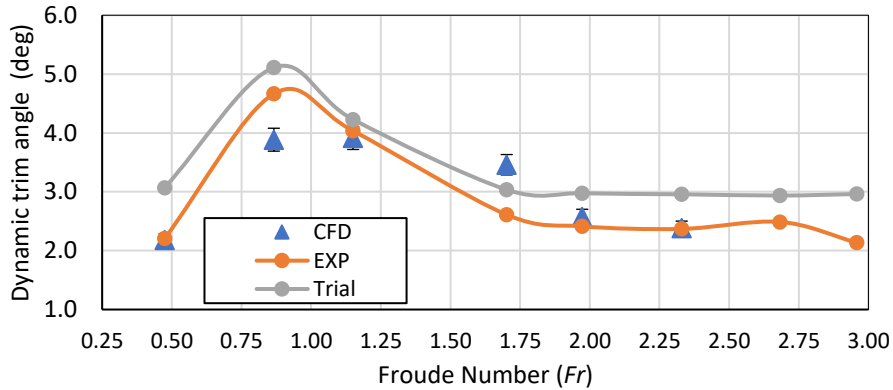
Figure 4. Dynamic trim angle comparison between experimental data, CFD (with uncertainty bar), and sea trial.
