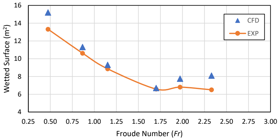
Figure 5. Dynamic wetted surface for full-scale CFD and full-scaled towing tank.
