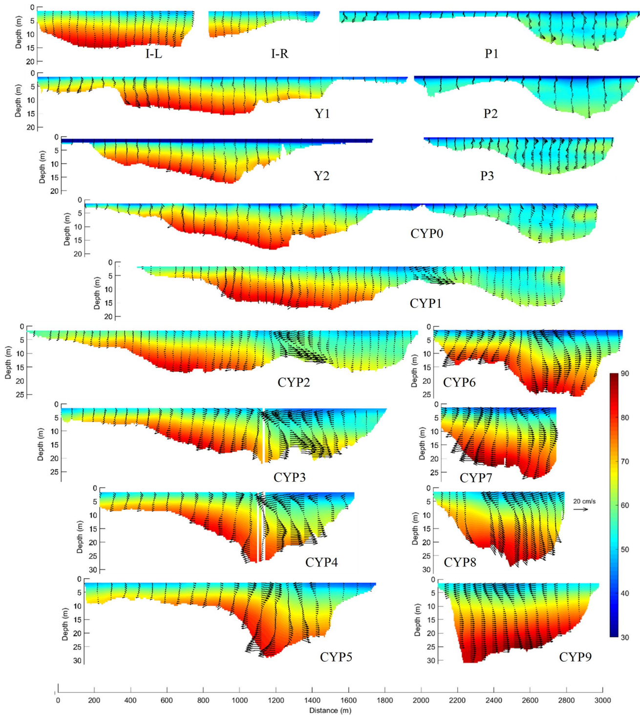
Figure 13. Spatial distribution of RB (representing suspended sediment concentration) in all cross sections in Survey 1 (Vector: secondary velocity; contour: RB).
