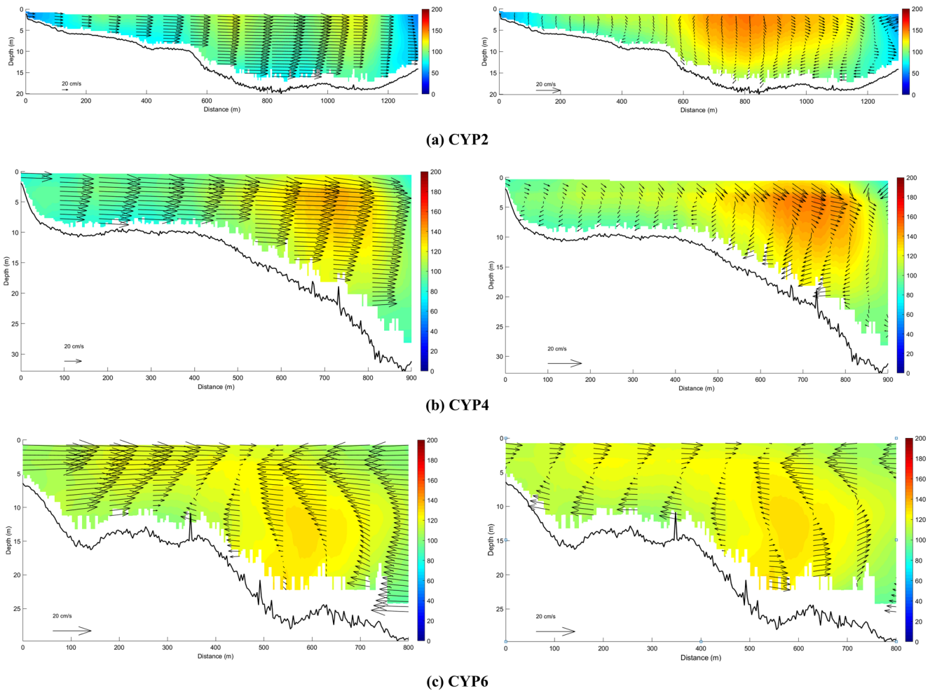
Figure 9. Raw data of velocity field (left image) and the rotated data by Rozovskii method (right image) at the left side of CYP2 (a), CYP4 (b), and CYP6 (c) in Survey 1, looking downstream (Vector: secondary velocity; contour: primary velocity with units of cm/s).
