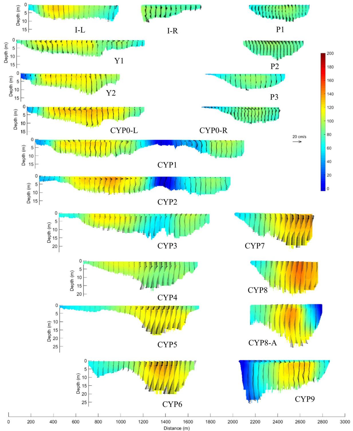
Figure 11. Secondary flows in all cross sections for the case in December Survey 2 (Vector: secondary velocity; contour: primary velocity with units of cm/s).
