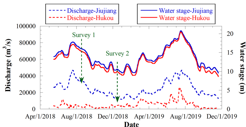
Figure 2. Annual variation of water level and flow discharge at Jiujiang and Hukou stations, and two surveys setup, one in the high flow conditions and the other in the low flow conditions, with a large difference on water level of about 5.8 m. The water level is according to the frozen base level whose zero datum is 1.91 m higher than that of 1985 National Height Datum.
