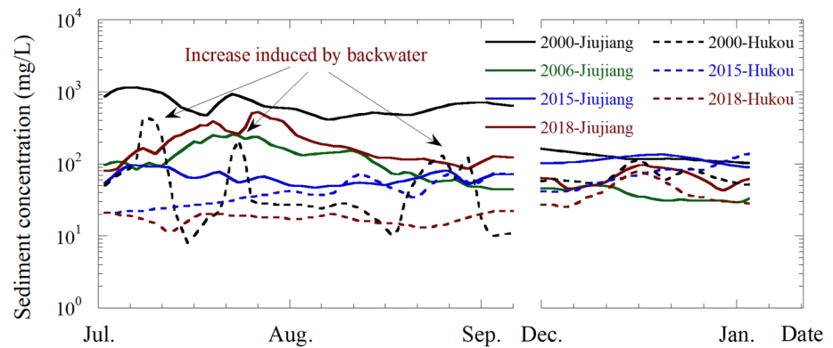
Figure 4. Sediment concentration at Jiujiang and Hukou hydrological stations before and after the operation of the Three Gorges Dam.
