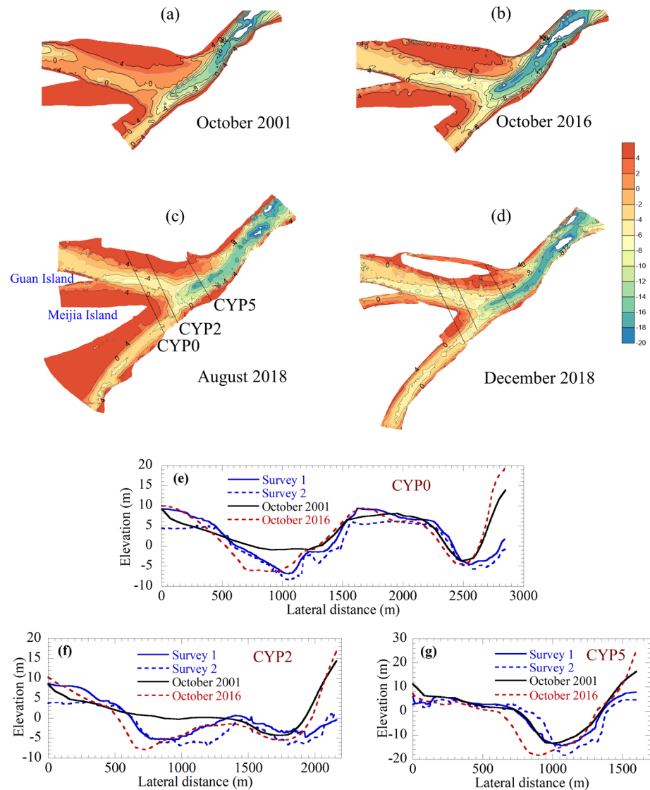
Figure 3. Bed elevations (water level minus water depth) of the confluence (with units of m) before the operation of the Three Gorges Dam in October 2001 (a), and after that in October 2016 (b), and Survey 1 (c), and Survey 2 (d). The contours of 2001 and 2016 were supplied by Bureau of Hydrology and Water Resources of the Lower Reaches of the Yangtze River; and contours of 2018 were calculated by the minus of the water level at Hukou Station and the water depth of the whole study site measured by ADCP. The profiles of the cross sectional bed surface at CYP0 (e), CYP2 (f), and CYP5 (g) are also plotted. Note that according to the water level difference between Jiujiang (about 19 km upstream of Hukou), Hukou, Anqing (about 129 km downstream of Hukou), the approximate water surface slope of this reach of the Yangtze River was 0.026‰ (Survey 2)~0.028‰ (Survey 1). That is, the difference of water level between upstream and downstream boundary (totally about 8 km long) was about 21 cm. The water level of the downstream boundary was 15.8 cm lower than that in Hukou, and that of the upstream boundary is 5.2 cm higher than that in Hukou. Comparing to the difference of bed elevation at different time, this difference of water level was neglected. Hence, only the water level at Hukou Hydrological Station was used to represent that of the whole study site.
