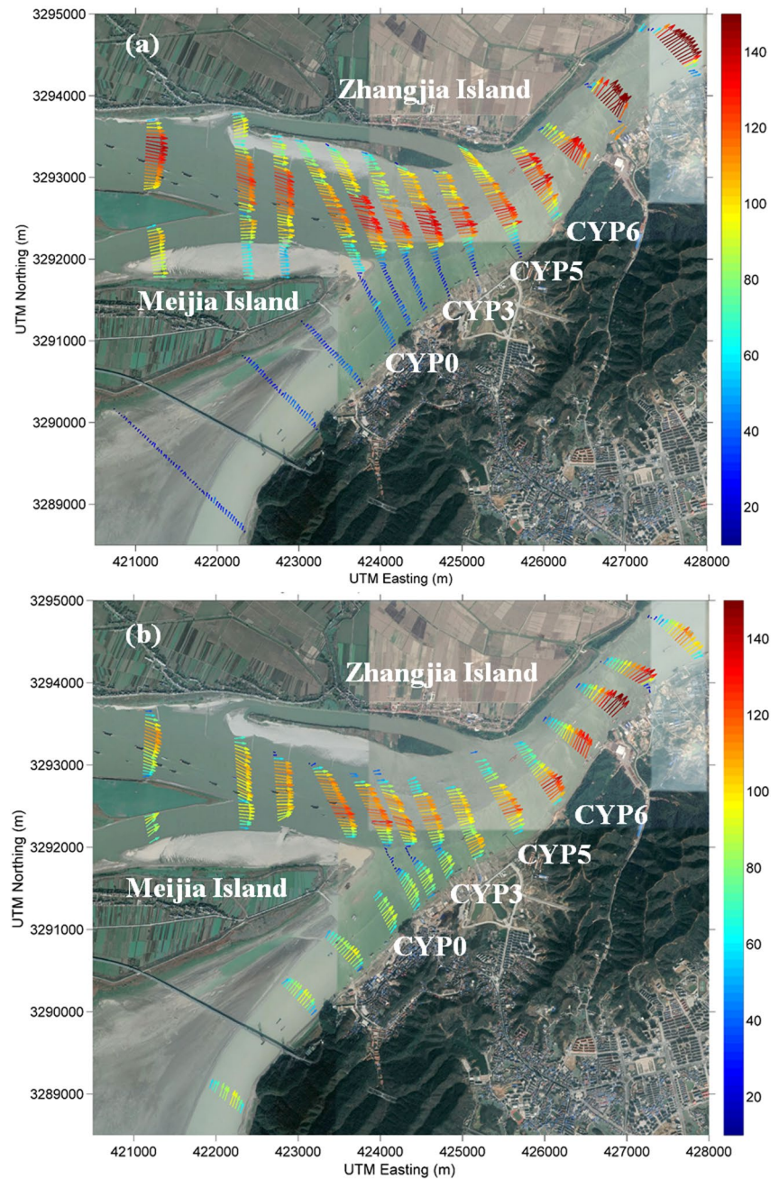
Figure 5. Vectors of vertically averaged flow velocities of Survey 1 (a) and Survey 2 (b) with units of cm/s.
