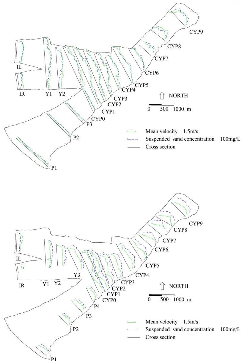
Figure 15. Depth-averaged suspended sediment concentration (represented by RB) and depth-averaged flow velocity at the confluence for two surveys.
