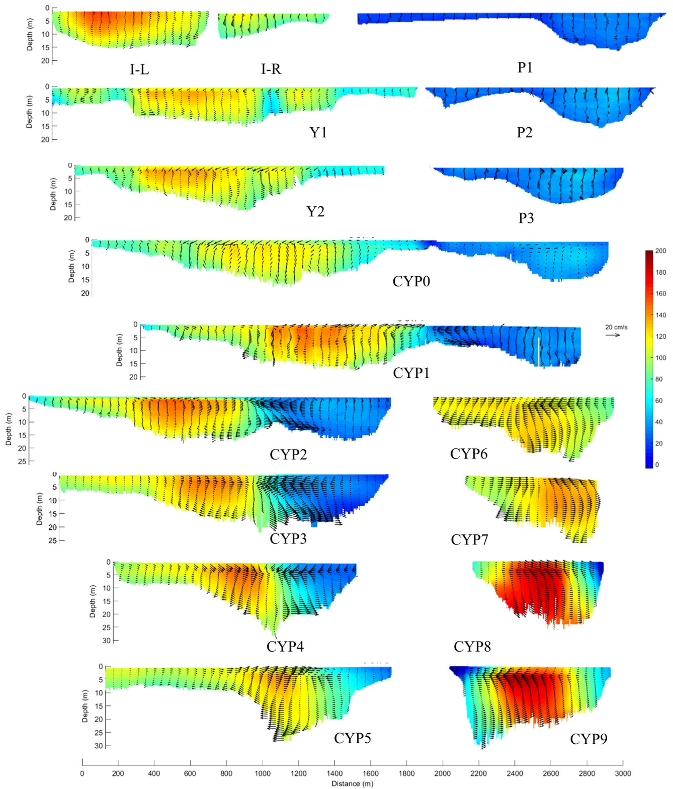
Figure 8. Secondary flows in all cross sections for the case in August Survey 1, looking downstream (Vector: secondary velocity; contour: primary velocity with units of cm/s).
