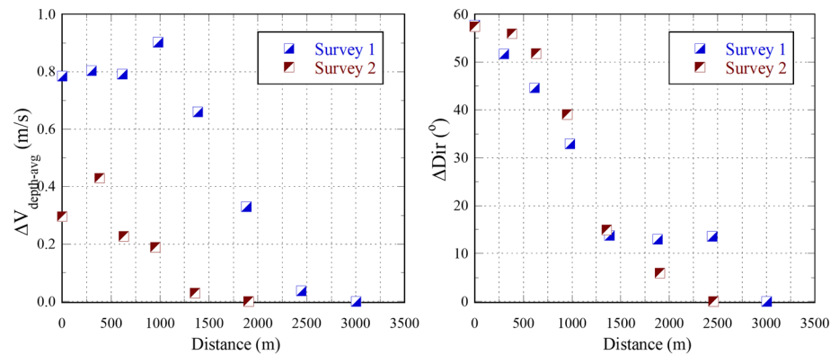
Figure 6. Difference in depth-averaged velocity magnitude ( \Delta V_{\text{depth-avg}} ; left image) and in flow direction ( \Delta \text{Dir} ; right image) between Yangtze River and Poyang Lake in two surveys. The horizontal axis shows the distance from the confluence apex near CYP0.
