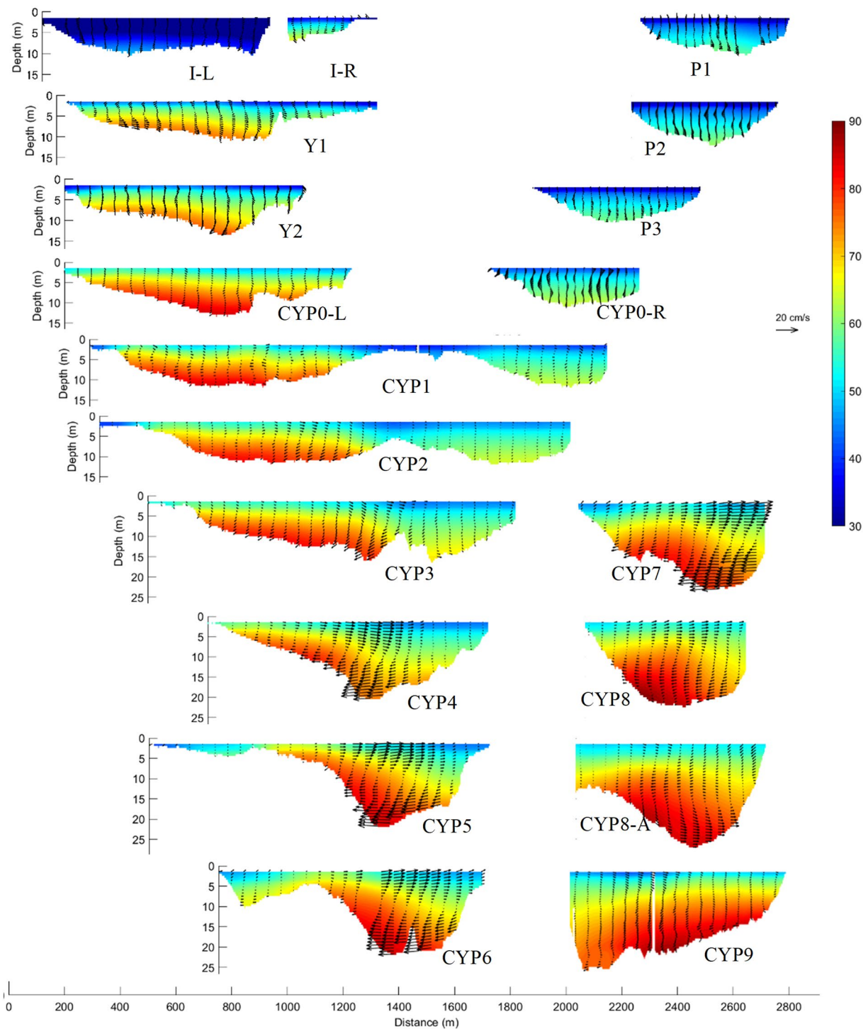
Figure 14. Spatial distribution of RB (representing suspended sediment concentration) in all cross sections in Survey 2 (Vector: secondary velocity; contour: RB).
