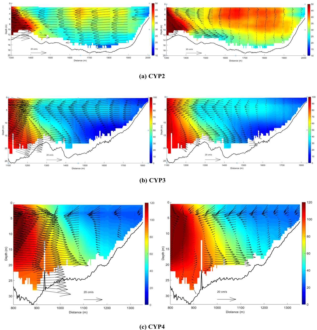
Figure 10. Raw data of velocity field (left image) and the rotated data by Rozovskii method (right image) at the right side of CYP2 (a), CYP3 (b), and CYP4 (c) in Survey 1, looking downstream (Vector: secondary velocity; contour: primary velocity with units of cm/s).
