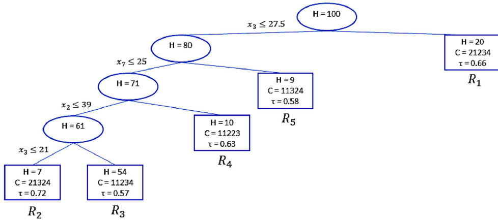
FIGURE 4. Pruned regression trunk: MS approach.
