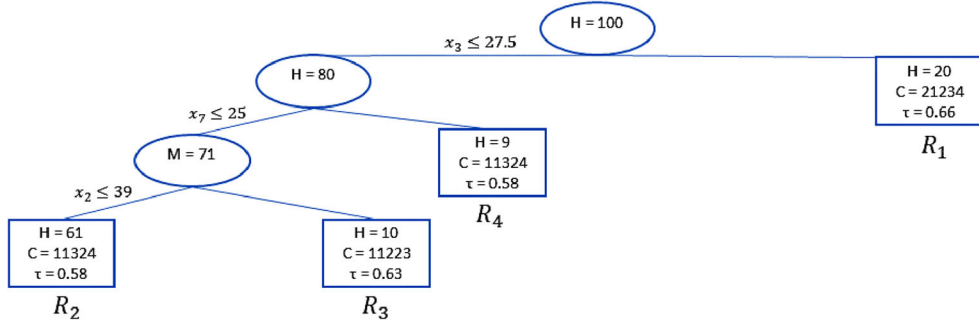
FIGURE 2. Pruned regression trunk: OSO approach.
