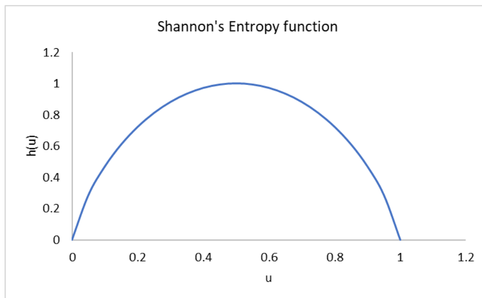
Figure 3. Shannon’s Entropy function.
