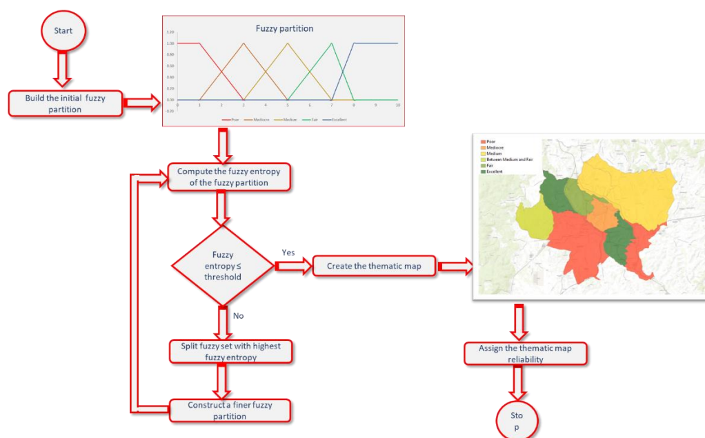
Figure 1. Schema of the Thematic Fuzzy Entropy Partition method (TFEP).
