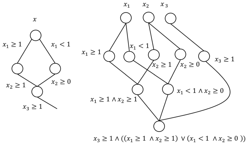
Figure 11: Example of transformation from a binary decision diagram to a neural network. For each edge in the binary decision diagram, we construct a depth-2 neural network node corresponding to the path from the root to the edge. Depth-1 neural network nodes correspond to edges in the binary decision diagram.
