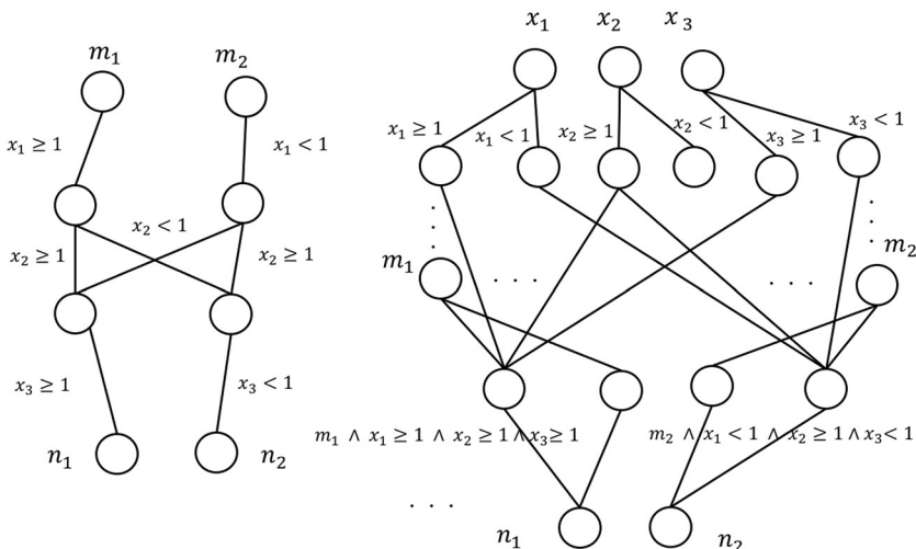
Figure 13: Example of transformation from a binary decision diagram to a neural network for b = 3 . Depth-1 nodes in the neural network correspond to edges in the binary decision diagram. For each path from m_1 or m_2 to n_1 or n_2 , we construct a corresponding neural network node.
