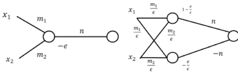
Figure 8: These two neural networks are equivalent. A constant on each edge is a weight, and weight zero edges are omitted. A constant near each node is a bias. The left neural network uses Heaviside activation functions, and the right neural network uses ReLU activation functions. \epsilon is a small, positive value. The left network represents nH(m_1x_1 + m_2x_2 - e) , and the right network represents n\text{ReLU}(m_1x_1/\epsilon + m_2x_2/\epsilon + 1 - e/\epsilon) - n\text{ReLU}(m_1x_1/\epsilon + m_2x_2/\epsilon - e/\epsilon) . These two expressions can be the same for the finite set of inputs if we use sufficiently small constant \epsilon > 0 .
