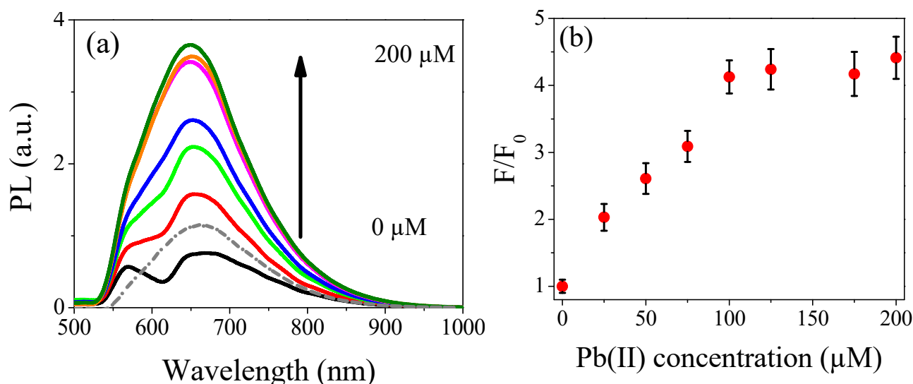
Figure 3. (a) PL spectra of the hydrogel matrix doped with AgNCs-PMAA as a function of Pb(II) concentration, the dotted grey line represents the emission of bare AgNCs-PMAA colloidal solution as reference; (b) the F/F_0 ratio as a function of Pb(II) concentration between 0–200 \mu\text{M} .
