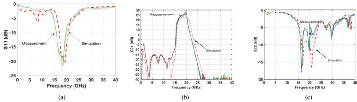
Fig. 17. Comparison between simulated (dash) and measured scattering parameters of 10 samples. (a) S_{11} , (b) S_{21} , and (c) S_{22} .
