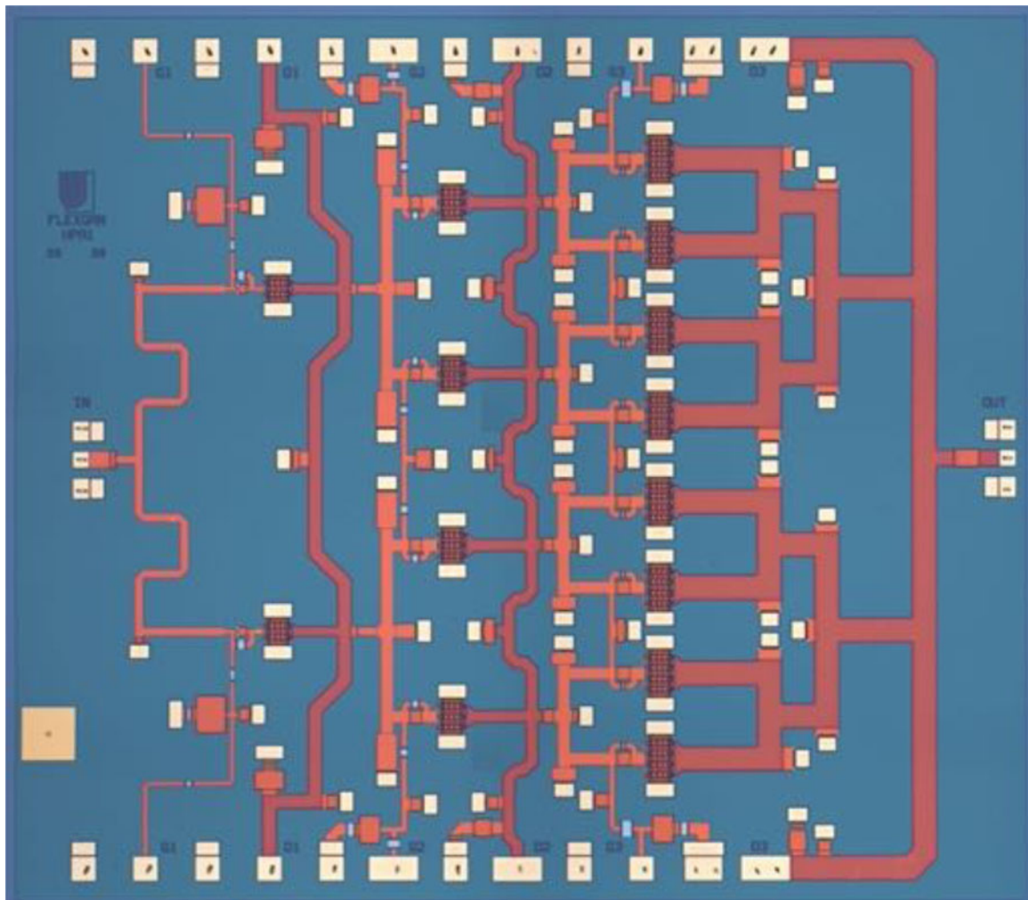
Fig. 12. Photo of the realized amplifier (size 5 \times 4.4 \text{ mm}^2 ).
