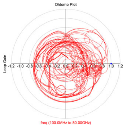
Fig. 11. Loop gain simulated by using the Ohtomo test [28], for the frequency from 100 MHz up to 80 GHz. The condition for stable loop is fulfilled if none of the loop gain encircles the point (1, 0) shown in the figure.
