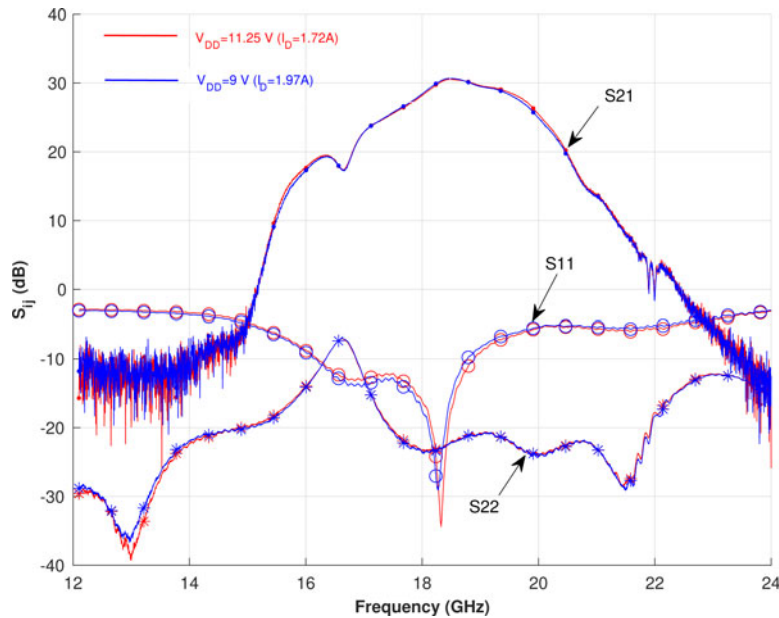
Fig. 20. Small-signal measured results in CW condition. The reference ports are the test-jig input/output RF ports (i.e., SMA connectors) and TRL calibration was considered.
