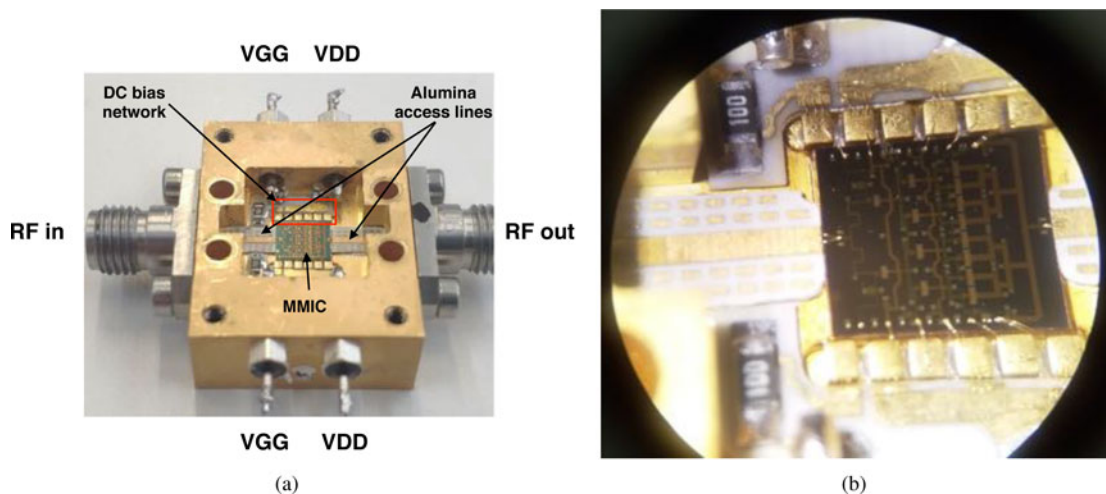
Fig. 19. (a) MMIC mounted in the package. (b) Zoom on the MMIC area.
