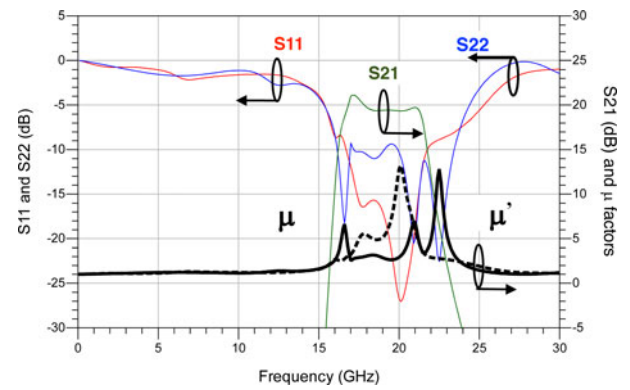
Fig. 13. Simulated small-signal S-parameter.
