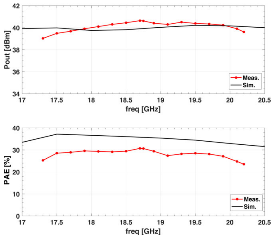
Fig. 21. Measured CW performance of the packaged MMIC (black lines are the simulation at MMIC level). The bias point is V_{DD}=11.25 V and total current absorption of 1 A, with P_{in}=15 dBm.
