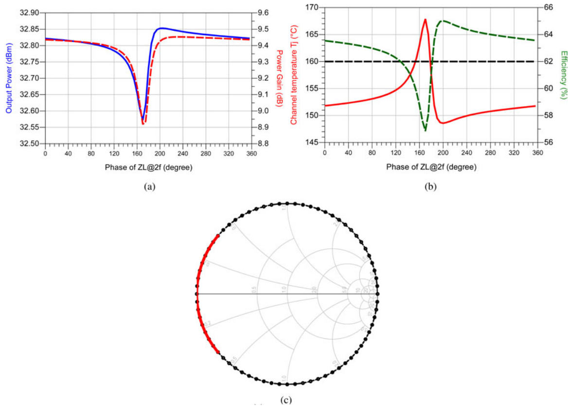
Fig. 3. Load-pull results performed with the fundamental frequency 18.75 GHz and P_m = 24.7 dBm and varying the phase of the second harmonic (37.5 GHz) for the 8 \times 100 \mu\text{m} device: (a) reports the simulated output power (blue curve, left axis) and power gain (red curve, right axis); (b) the corresponding estimated channel temperature (red curve, left axis) and power added efficiency (green curve, right axis); (c) the loading condition assumed at 37.5 GHz, are represented by the black points, while the critical region to be avoided is represented by the red circles. (a) Output power and gain, (b) efficiency and junction temperature, and (c) critical area.
