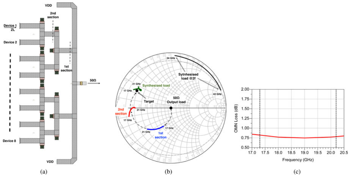
Fig. 6. Designed output combiner (a) and synthesized load (b). The power losses result in \sim 0.8 dB (c). (a) Output combiner. (b) Synthesized loads. (c) Combiner loss.
