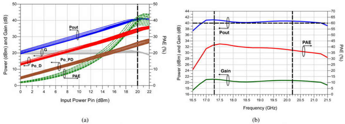
Fig. 14. Simulated performance: (a) as a function of the input power for the carrier frequencies from 17.3 to 20.2 GHz; (b) over frequency for a fixed input power level P_{in} = 20 dBm. (a) Power sweep. (b) Frequency sweep.
