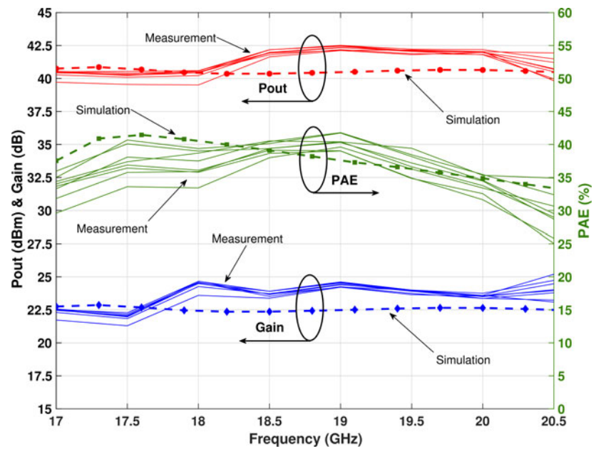
Fig. 18. Comparison between simulated (dashed lines) and measured (continuous lines) power performances. The latter refers to the same MMIC version located in different wafer positions, to test the reproducibility of the results on the wafer.
