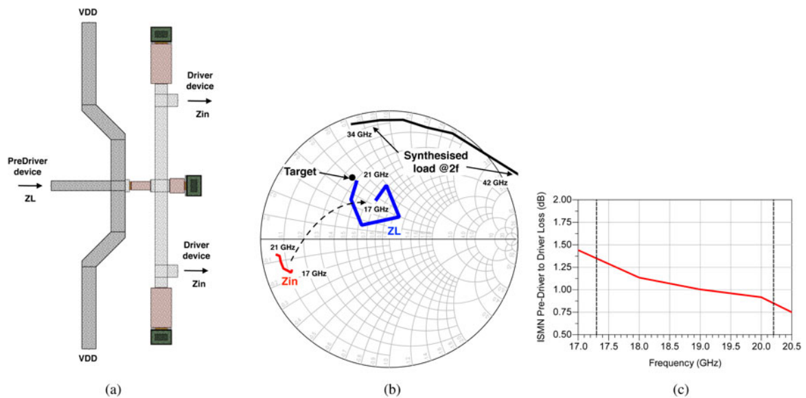
Fig. 10. Designed interstage matching network from one pre-driver to two driver devices (a) and synthesized load (b). The power losses result within 0.8-1.3dB (c). (a) Interstage matching network between one pre-driver and two driver devices. (b) Synthesized loads. (c) Combiner loss.
