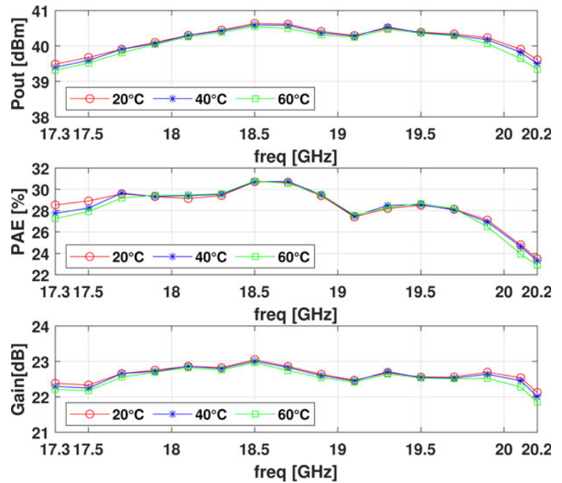
Fig. 22. Measured CW performance of the packaged MMIC at the nominal bias point and for different temperatures.
