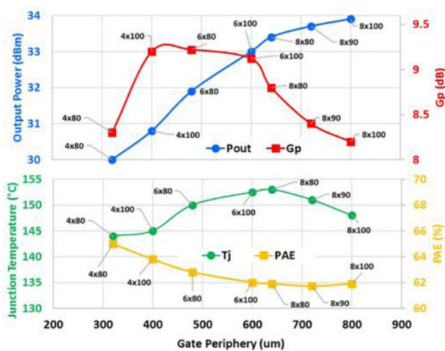
Fig. 4. Output power, associated gain, and PAE at 2 dB of gain compression together with the correspondent channel temperature T_j , simulated at center frequency 18.75 GHz for different device geometries.
