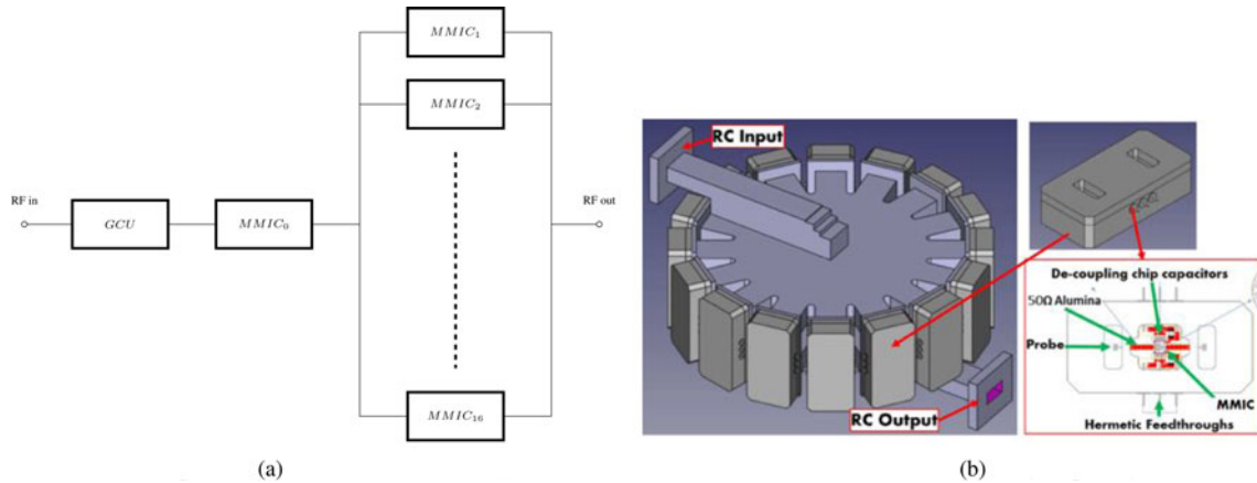
Fig. 1. Schematic architecture of the SSPA. (a) Simplified scheme of the SSPA RF tray. (b) Radial combiner solution integrating 16 packaged MMICs.
