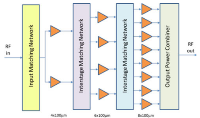
Fig. 5. Architecture of the HPA MMIC. For the networks, it has been preliminary estimated a power loss of 1 dB for the output combiner and 1.5 dB for both the interstage matching networks.
