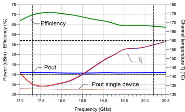
Fig. 7. Simulated performance of the final stage alone, when each device is driven with 24 dBm of input power at its gate.
