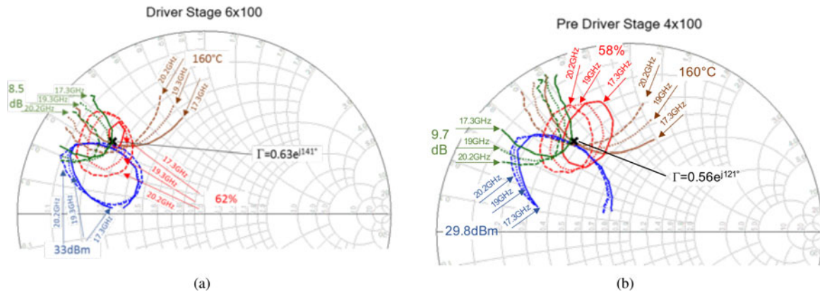
Fig. 8. Simulated load pull for the devices used in the driver (a) and pre-driver (b) stages. The former is 6 \times 100 \mu\text{m} , the latter 4 \times 100 \mu\text{m} , both biased with V_{D0}=11.25\text{ V} and quiescent current I_{D0}=27\text{ mA} and I_{D0}=18\text{ mA} , respectively. The contour plots refer to 1 dB of gain compression.
