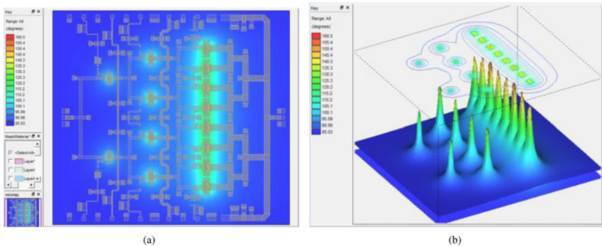
Fig. 16. Simulated thermal map of the designed MMIC, assuming T_{BP} = 85^\circ\text{C} and for the overall stack (below MMIC) a thermal resistance R_{th,stack} = 0.28^\circ\text{C/W} . (a) Two-dimensional view at MMIC level; (b) Three-dimensional view to see the temperature spread in the vertical section.
