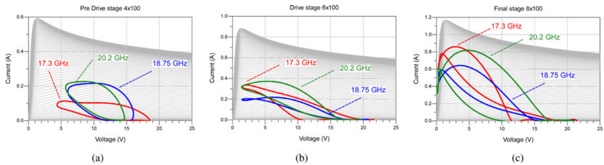
Fig. 15. Load lines for the devices in the pre-driver (a), driver (b), and final stages (c), respectively, simulated for P_{in} = 20 dBm.
