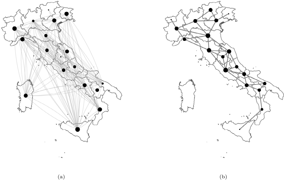
Fig. 2. Network structure of the two adjacency matrices considered: \mathbf{W}_1 (a) and \mathbf{W}_2 (b).
