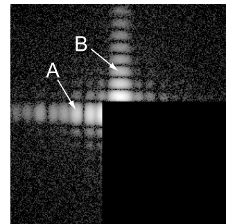
Figure 2. Coherent x-ray diffraction pattern of the test structure in 301 \times 301 pixels.
