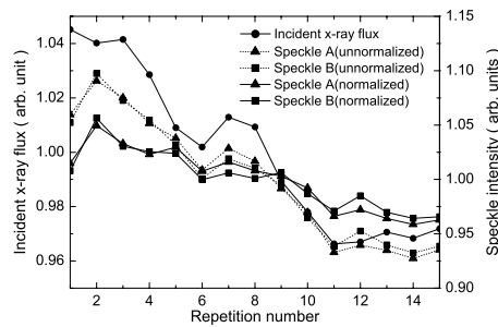
Figure 3. Repetition number dependence of the incident x-ray flux and intensities of speckles shown by arrows in Fig. 2. Each plot was normalized by the average value of 15 data. Speckle intensities shown by solid lines were normalized by the incident x-ray flux.
