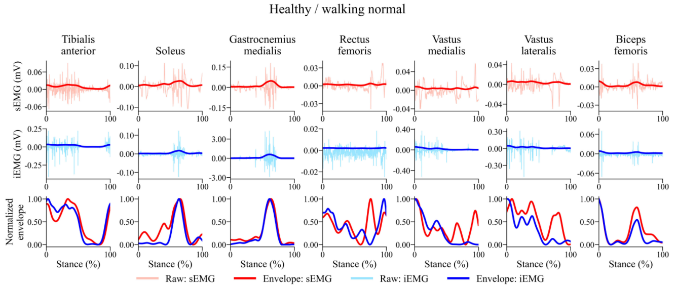
Fig. 9. Representative surface and intramuscular EMG measurements from a healthy subject's walking trial.
