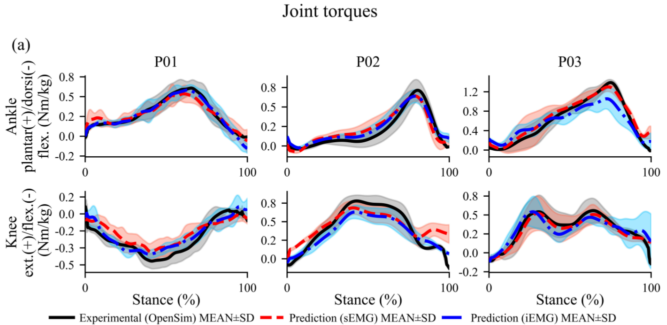
Fig. 6. Joint torque estimation results using the EMG-driven modeling framework for all iSCI subjects. Black lines show the mean of the experimental (reference) joint torques evaluated by inverse dynamics analysis in OpenSim. Red lines show the mean of the predicted joint torques using sEMG whereas blue lines show the mean of the predicted joint torques using iEMG. The shaded area shows 1 standard deviation (SD) for each time step during the entire stance phase of walking trials. For each subject, 7 trials were used for the execution of the NMS model.
