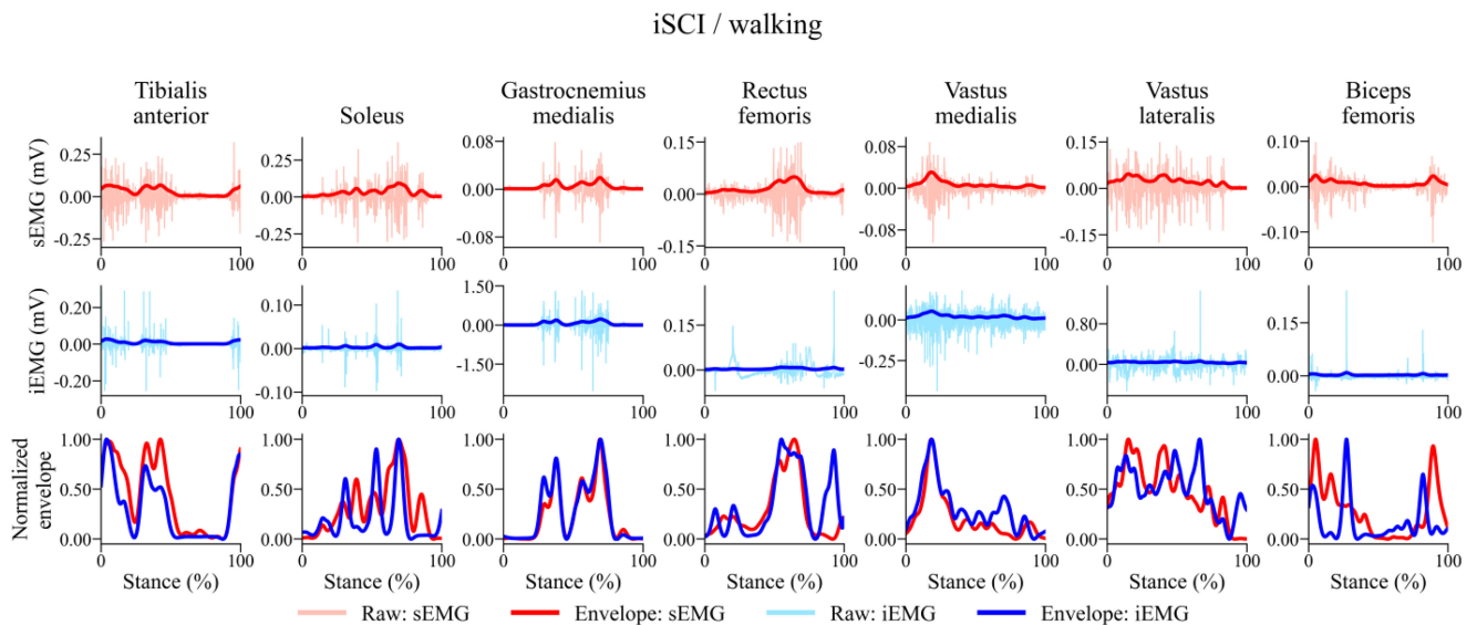
Fig. 10. Representative surface and intramuscular EMG measurements from an iSCI subject's walking trial.
