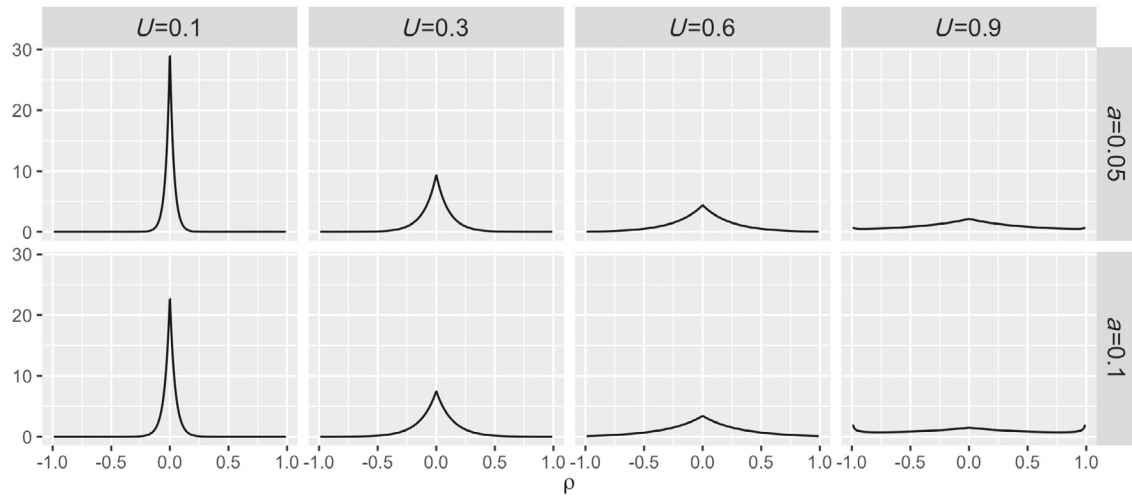
FIGURE 2 Prior densities for \rho using a PC-prior with \rho_0 = 0 , c = 2 and different values for U and a
