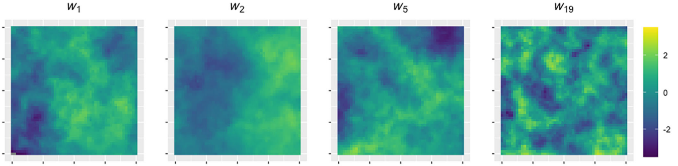
FIGURE 3 The PCA variables w_1 , w_2 , w_5 , and w_{19} , associated with eigenvalues index 1, 2, 5, and 19
