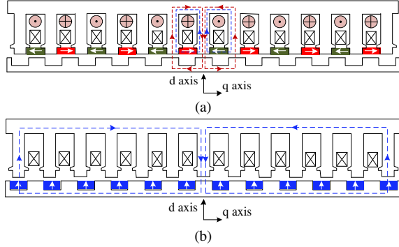
Fig. 10. D-axis flux for two structures. (a) RDCS-RM. (b) CP-VPMM.
