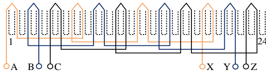
Fig. 3. Connection of the armature winding.
