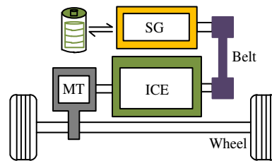
Fig. 1. Configuration of BSG system in HEV. (MT—mechanical transmission, ICE—internal combustion engine, SG—starter-generator).
