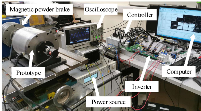
Fig. 21. Experiment setup.
