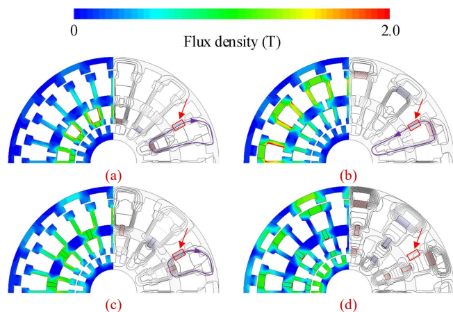
Fig. 7. Open-circuit flux distribution. (a) With only inner slot PMs. (b) With only outer slot PMs. (c) With only yoke PMs. (d) With all PMs.
