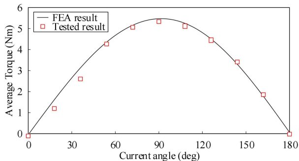
Fig. 23. Tested output torque and simulated electromagnetic torque.
