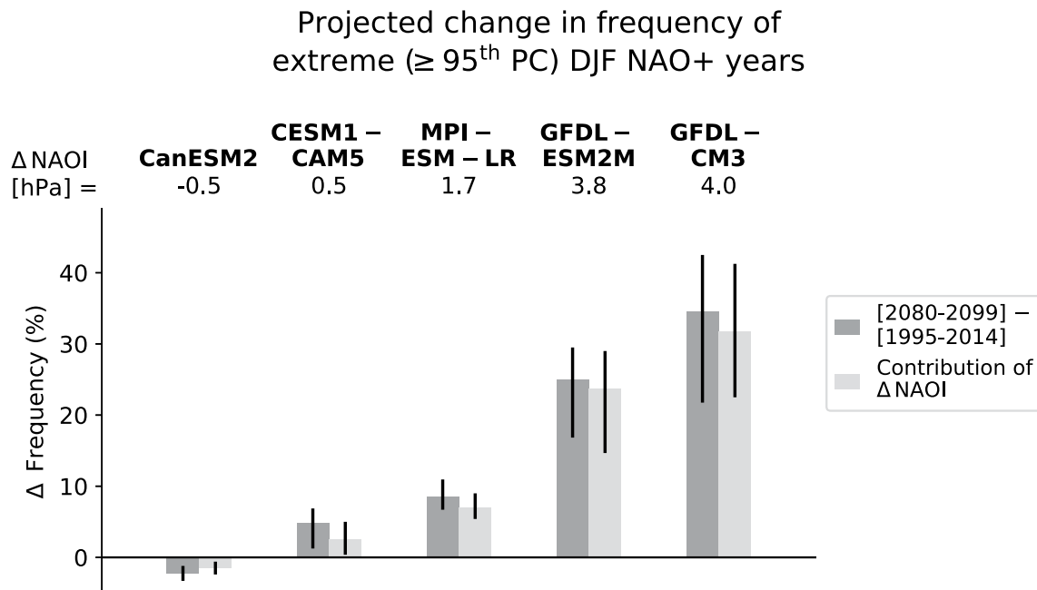
Figure 2. Projected change (2080–2099 minus 1995–2014) in the frequency of extreme positive ( \geq 95^{\text{th}} percentile for 1995–2014) North Atlantic Oscillation (NAO) winters for selected Multimodel Large Ensemble Archive (MMLEA) models (see Section 3.1). Contribution of mean December to February (DJF) NAO index change ( \Delta \text{NAOI} ) is calculated by shifting the 1995–2014 distribution of annual DJF NAO index by \Delta \text{NAOI} . Error bars show bootstrapped 95% confidence intervals.
