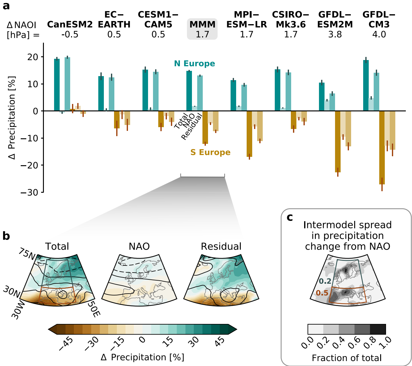
Figure 1. Role of forced December to February (DJF) North Atlantic Oscillation (NAO) index change ( \Delta NAOI) in DJF precipitation projections (2080–2099 minus 1995–2014) for the Multimodel Large Ensemble Archive (MMLEA) models. (a) Area-average precipitation anomalies in northern (blue) and southern (brown) Europe; regions are defined by blue and brown boxes in (b). Left bar: Total anomaly; Middle bar: NAO-congruent part; Right bar: Residual. Precipitation anomalies are shown as a percentage of the 1995–2014 climatology. Error bars show bootstrapped 95% confidence intervals. (b) Maps of multimodel mean (MMM) precipitation (shading) and mean sea level pressure (contours) anomalies; Figure S5 in Supporting Information S1 shows maps for each model. Contours range from -2 hPa (dashed) to 2 hPa (solid) in 1 hPa intervals. (c) Fraction of total intermodel variance in precipitation projections that is NAO-congruent; see Figure S6 in Supporting Information S1 for further explanation. Colored numbers indicate fractions for northern and southern European precipitation changes in (a).
