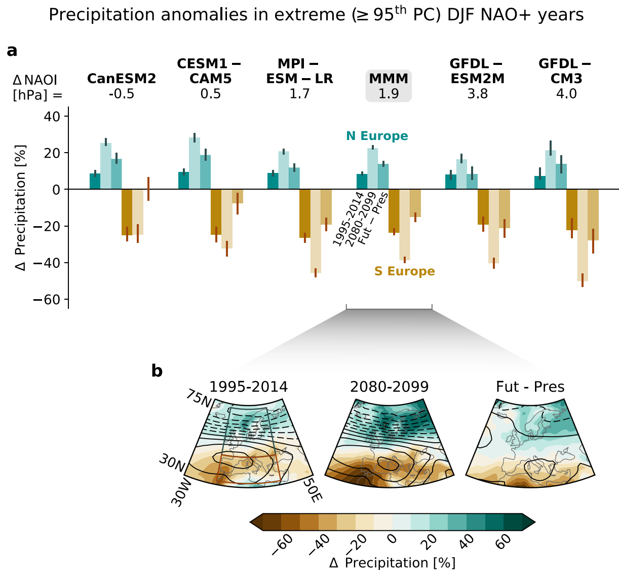
Figure 3. Precipitation anomalies during extreme positive ( \geq 95^{\text{th}} percentile) NAO winters for 2080–2099 versus 1995–2014 in selected Multimodel Large Ensemble Archive (MMLEA) models (see Section 3.1). (a) Area-average precipitation anomalies in northern (blue) and southern (brown) Europe; regions are defined by blue and brown boxes in (b). Left bar: 1995–2014 anomaly; Middle bar: 2080–2099 anomaly; Right bar: 2080–2099 anomaly minus 1995–2014 anomaly. Precipitation anomalies are shown as a percentage of the 1995–2014 climatology and averaged over all extreme positive NAO winters. Error bars show bootstrapped 95% confidence intervals. \Delta \text{NAOI} is the mean DJF NAO index change for 2080–2099 minus 1995–2014. The multimodel mean (MMM) is for the selected models only. (b) Maps of MMM precipitation (shading) and mean sea level pressure (contours) anomalies; Figure S9 in Supporting Information S1 shows maps for each model. Contours range from -10.5 hPa (dashed) to 6 hPa (solid) in 1.5 hPa intervals.
