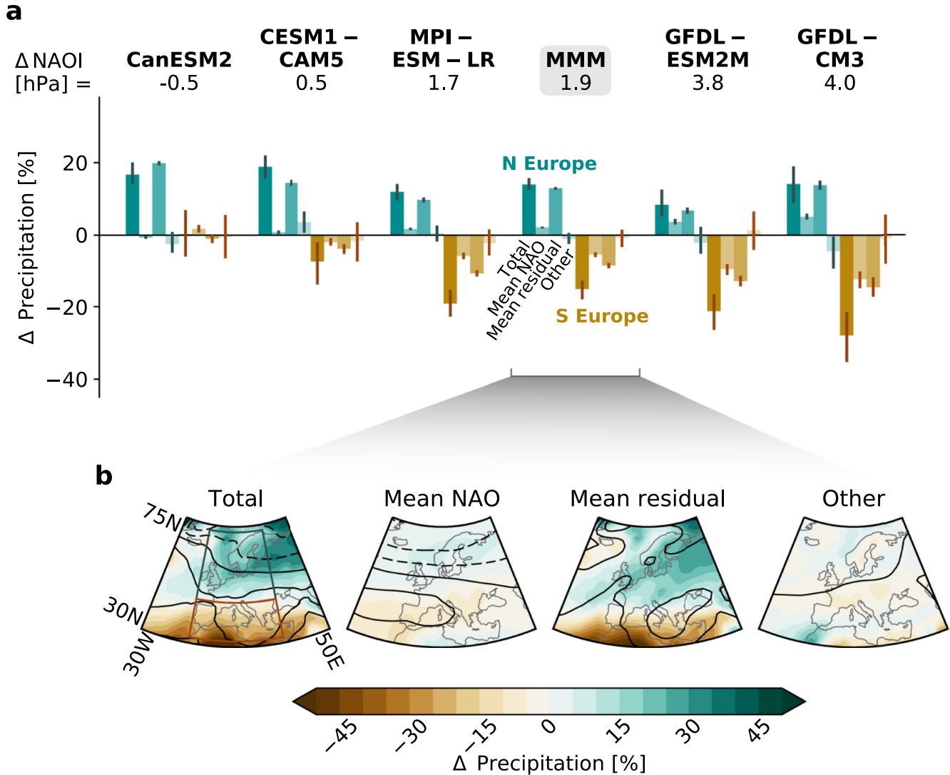
Figure 4. Decomposition of projected precipitation change (2080–2099 minus 1995–2014) during extreme positive ( \geq 95^{\text{th}} percentile) NAO winters in selected Multimodel Large Ensemble Archive (MMLEA) models (see Section 3.1). (a) Area-average precipitation anomalies in northern (blue) and southern (brown) Europe; regions are defined by blue and brown boxes in (b). Far left bar: Total anomaly; Middle left bar: Part from mean DJF NAO index change ( \Delta \text{NAOI} , NAO part in Figure 1); Middle right bar: Part from mean residual change (residual in Figure 1); Far right bar: Non-climatological “other” part. Precipitation anomalies are shown as a percentage of the 1995–2014 climatology and averaged over all extreme positive NAO winters. Error bars show bootstrapped 95% confidence intervals. The multimodel mean (MMM) is for the selected models only. (b) Maps of MMM precipitation (shading) and mean sea level pressure (contours) anomalies. Contours range from -2 hPa (dashed) to 1 hPa (solid) in 1 hPa intervals.
