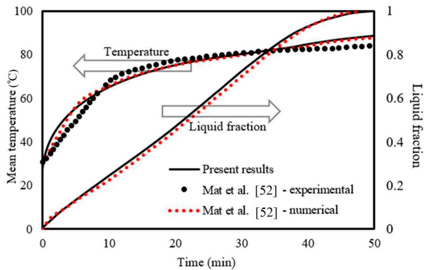
FIGURE 5 Evaluation of the current model's temperature and liquid-fraction results compared to those of Mat et al. (2013).
