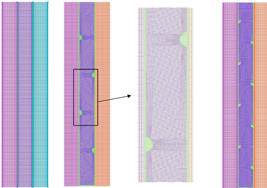
FIGURE 4 Schematic of the mesh for the cases of no-fin, staggered hemispherical fins, and staggered quarter spherical fins with an added fin.
