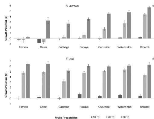
Figure 1. S. aureus (A) and E. coli (B) growth potential ( \alpha ) on fruits and vegetables at 10, 20 and 30 °C.
