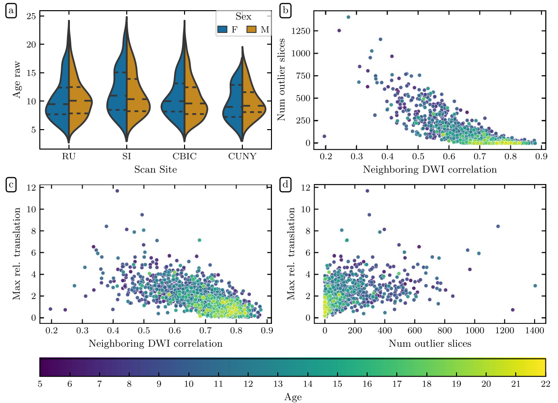
Fig. 10 Demographic and QSIprep quality metric distributions: (a) HBN age distributions by sex for each scanning site. Dashed lines indicate age quartiles. The remaining plots show associations between (b) neighboring diffusion-weighted imaging (DWI) correlation 17 and the number of outlier slices, (c) neighboring DWI correlation and maximum relative translation, and (d) the number of outlier slices and maximum relative translation. The number of outlier slices is positively associated with the maximum relative translation, while neighboring DWI correlation is negatively associated with the other two metrics. These plots are colored by age, and reveal that older participants generally have higher quality data.
