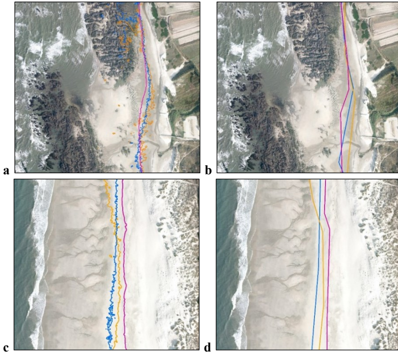
Fig. 2: Shoreline positions at two different beaches: the 1.05 m isolines of the 2011 DTM (pink), 2017 DEM (blue) and 2018 DEM (orange) (a, c) and the simplified shoreline used for the analyses (b, d).
