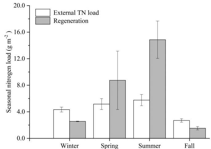
Fig 6. Mean seasonal TN loading and extrapolated internal whole-lake NH 4 + regeneration load in Lake Taihu.
