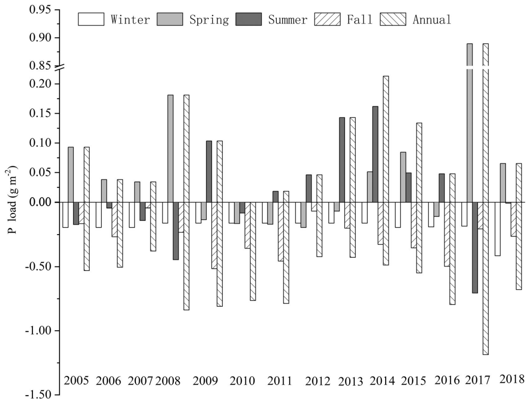
Fig 7. Seasonal and annual P release and burial for 2005–2018. Positive values indicate net P release. Negative values indicate net burial.
