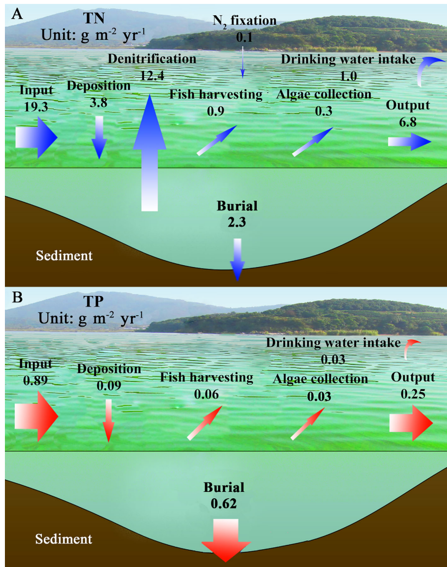
Fig 8. Diagrammatic presentation of TN (total nitrogen; panel A) and TP (total phosphorus; panel B) budgets for Lake Taihu. [Corrections added on 22 March 2021, after first online publication: Units changed from \text{g.m}^{-2} \cdot \text{year}^{-1} to \text{g m}^{-2} \text{ yr}^{-1} .]
