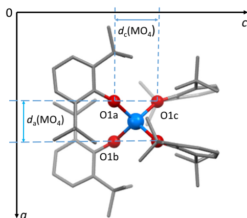
Fig. 2 | The structure of Np(OAr) 4 in the solid state at ambient pressure.
