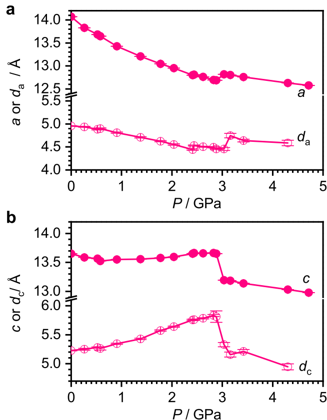
Fig. 3 | The effect of pressure on selected crystallographic metrics of Th(OAr) 4 . a Solid circles: the length of the unit cell parameter a (=b) as a function of pressure. Open circles: the projected contribution of the ThO 4 moiety to the a axis length. b Corresponding plots for the c axis. Similar plots for U(OAr) 4 and Np(OAr) 4 are available in Supplementary Figs. 8 and 9. Calculation of the projected dimensions and their error bars is explained in the Supplementary Information, Section 1.17.
