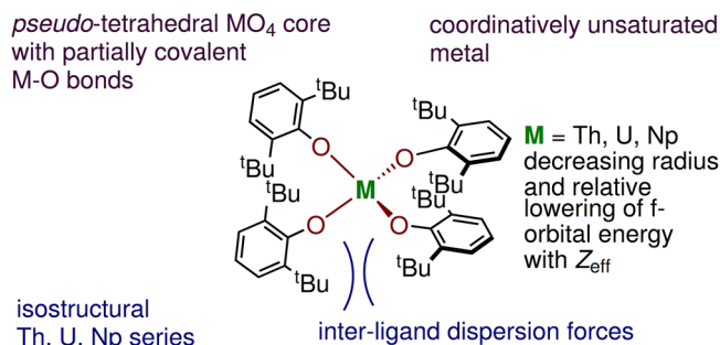
Fig. 1 | Pseudo tetrahedral actinide molecules investigated in this study. Chemical structure of tetra-coordinated early actinide aryloxides M(OAr) 4 (M = Th, U, Np; OAr = 2,6-di- tert -butylphenoxide).
