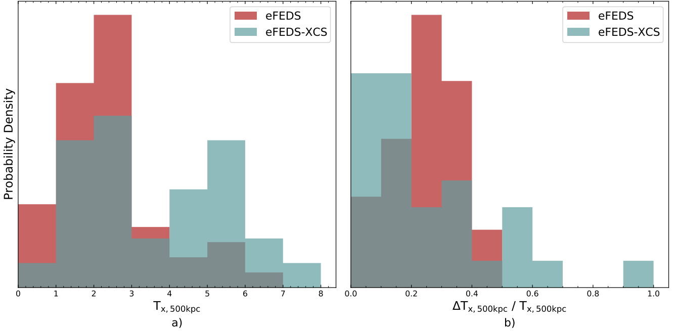
Figure 11. Temperature and fractional temperature error distributions of the eFEDS (red) and eFEDS-XCS (pale blue) samples, for measurements made within 500 kpc apertures, centered on eFEDS coordinates. The eFEDS sample plotted in red contains 95 eROSITA temperature measurements, and the eFEDS-XCS sample plotted in pale blue contains 28 XMM temperature measurements.
