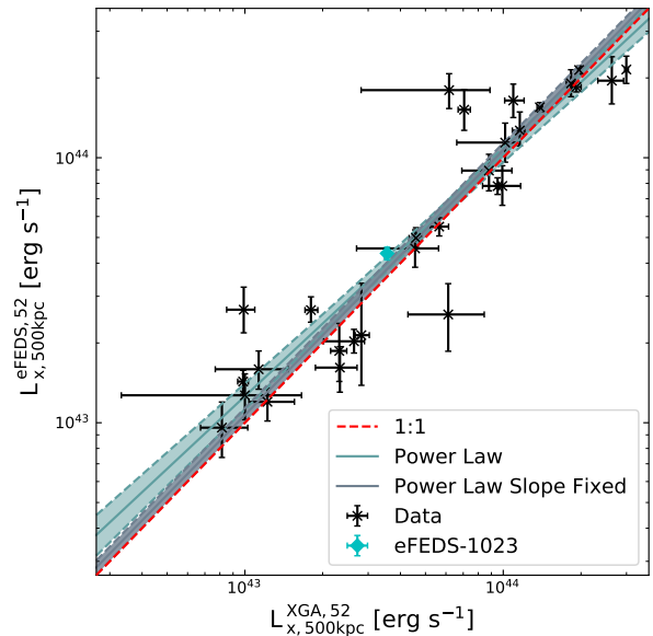
Figure 10. Comparison of unabsorbed cluster luminosities within a 500 kpc aperture, in the 0.5-2.0 keV energy band, centered on eFEDS coordinates. Pale blue line indicates best fit power-law, with 68% confidence levels given by shaded region. Grey line indicates a power-law fit with slope set to 1 (with 68% confidence levels given by grey shaded region). Cyan diamond is for the split cluster discussed in Appendix B.
