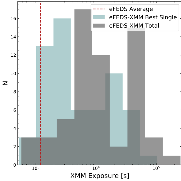
Figure 3. Distribution of exposure times for eFEDS-XMM cluster candidates, measured at the eFEDS coordinates. Exposures taken from 0.5-2.0 keV exposure maps, corrected for flaring and vignetting. Dashed line indicates the average vignetting corrected exposure of the eFEDS field reported by Liu et al. (2021a).
