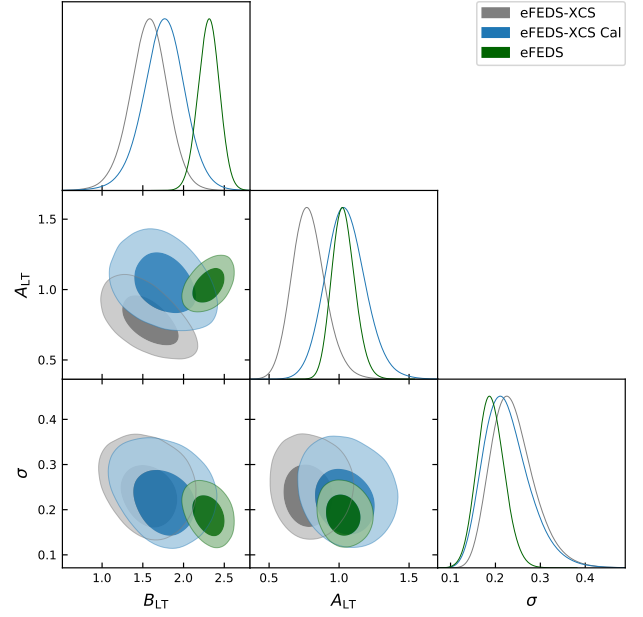
Figure 14. Corner plot of the 1\sigma and 2\sigma confidence contours of the L_{X, 0.5-2.0}^{500kpc} - T_{X, 500kpc}^{500kpc} relation parameters, for the eFEDS (green contours), eFEDS-XCS (grey contours) and eFEDS-XCS calibrated (blue contours) samples. The diagonal shows the posterior densities of each parameter.
