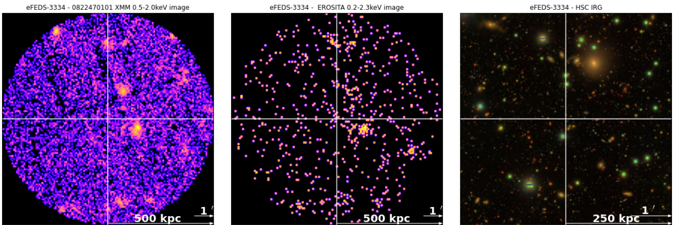
Figure 6. eFEDS- XMM cluster candidate (eFEDS ID 3334) without an obvious corresponding source of emission (see Section 3.3.2). The cross-hair indicates the eFEDS position. Left hand side is a combined PN+MOS1+MOS2 XMM image (ObsID 0822470101), centre is eROSITA , right hand side is HSC. Both XMM and eROSITA images are cutouts within a radius of 500 kpc, HSC image has a smaller half-side-length of 250 kpc (at the redshift provided by eFEDS).
