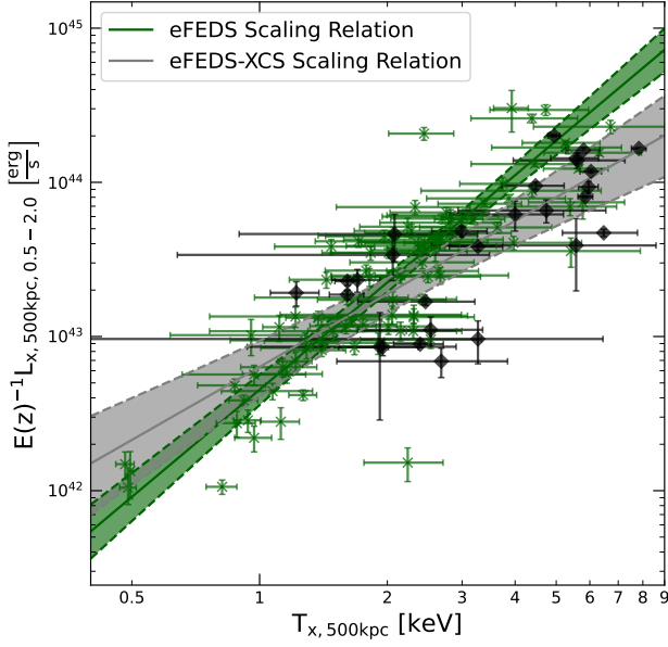
Figure 13. Soft-band (0.5-2.0 keV) luminosity-temperature relations for the eFEDS and eFEDS-XCS samples. Properties measured within a 500 kpc fixed aperture centered on the eFEDS positions. eFEDS data points are green crosses and the model fit is green, eFEDS-XCS data points are black diamonds with a grey model fit.
