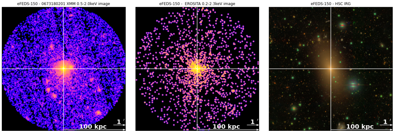
Figure 9. A low redshift eFEDS- XMM cluster candidate (eFEDS ID 150) whose X-ray emission is dominated by an X-ray bright elliptical galaxy (see Section 3.4). Left hand side is a combined PN+MOS1+MOS2 XMM image (ObsID 0673180201), centre is eROSITA , right hand side is HSC. Both XMM and eROSITA images are cutouts within a radius of 100 kpc, HSC image has a half-side-length of 100 kpc (at the redshift provided by eFEDS).
