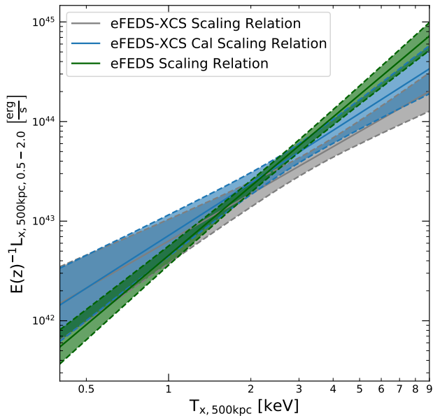
Figure 15. Soft-band luminosity-temperature relations for eFEDS, eFEDS-XCS, and calibrated eFEDS-XCS. Properties measured within a 500 kpc fixed aperture centered on the eFEDS positions.
