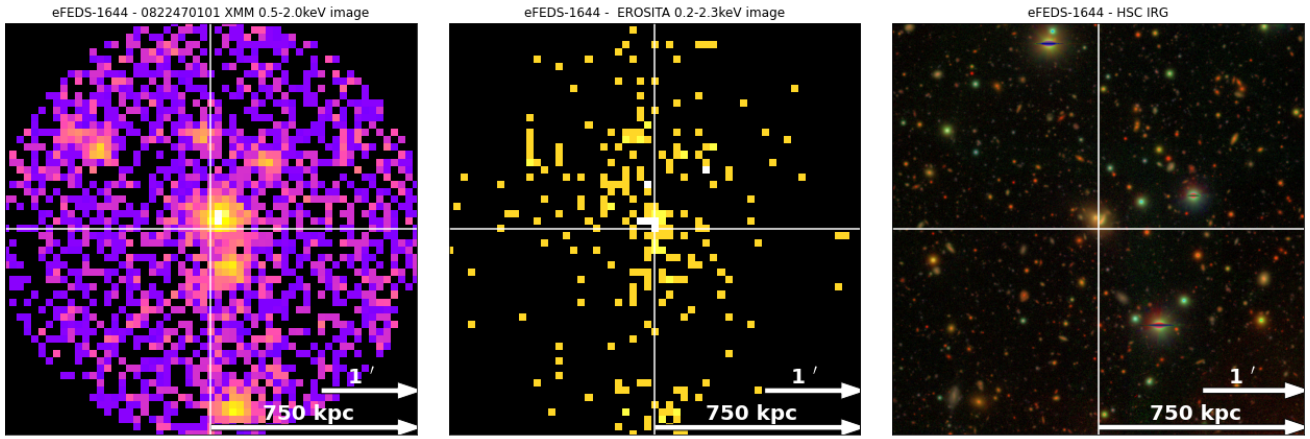
Figure 5. eFEDS- XMM cluster candidate (eFEDS ID 1644) identified as a pair interacting galaxies with ongoing AGN activity (see Section 3.3.1). The cross-hair indicates the eFEDS position. Left hand side is a combined PN+MOS1+MOS2 XMM image (ObsID 0822470101), centre is eROSITA , right hand side is HSC. Both XMM and eROSITA images are cutouts within a radius of 750 kpc, HSC image has a half-side-length of 750 kpc (at the redshift provided by eFEDS).
