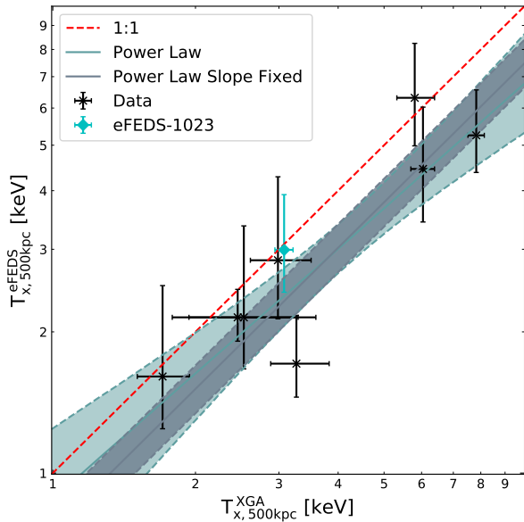
Figure 12. Comparison of eFEDS and XCS cluster temperatures within 500 kpc, centered on eFEDS coordinates. Pale blue line indicates best fit power-law (slope free to vary), with 68% confidence levels given by shaded region. Grey line indicates a power-law fit with fixed slope of unity (with 68% confidence levels given by the grey shaded region). Cyan diamond is for the split cluster discussed in Appendix B.
