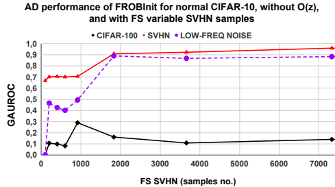
Figure 3: Performance of FROBInit in GAUROC for normal CIFAR-10 w/o O(\mathbf{z}) and w/ variable number of FS samples from SVHN.
