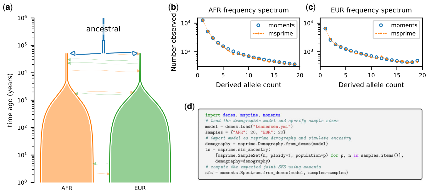
Fig. 2. Illustration and simulation using Demes. a) Using an inferred demographic model from Tennessen et al. (2012) specified as a YAML file in Demes format ( Fig. A2 ), we used demesdraw to visualize the demographic model (note the recent exponential growth resulting in present-day population sizes that greatly exceed those in the past). We then used msprime to simulate genomic data for 20 genome copies sampled from the two contemporary populations, and we used moments to compute the expected joint site-frequency spectrum for the same sample sizes ( Fig. A3 ). b, c) We compared the single-population SFS in each population, showing agreement between the simulation methods. d) Python code snippets of the interactions between demes and the simulation software. An extended script to compute the SFS shown in (b) and (c) is given in Fig. A3 .
