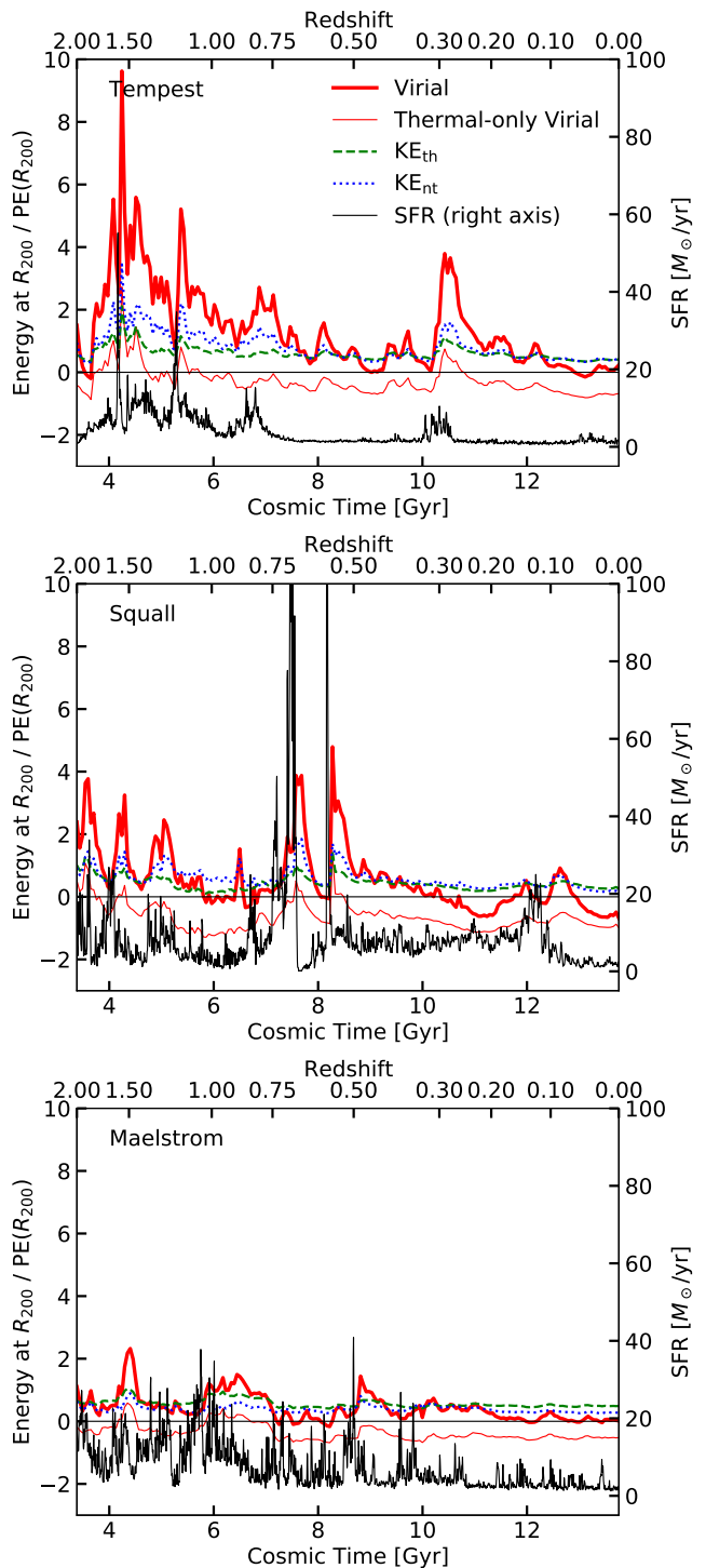
Figure 3. Energies of the gas within 0.99R_{200} < r < R_{200} as a function of cosmic time (bottom axis) and redshift (top axis). All energies are normalized by \frac{GM_{200}}{R_{200}} . The virial energy (Eq. 9) is plotted as the thick red line. The thermal kinetic energy of the gas is plotted as the green dashed line and the non-thermal kinetic energy is plotted as the blue dotted line. A thin solid red line indicates the virial energy of the gas near R_{200} if KE_{nt} is neglected in the virial equation. The SFR of the central 20 kpc of the halo is shown as the thin black line, with values indicated on the right axis.
