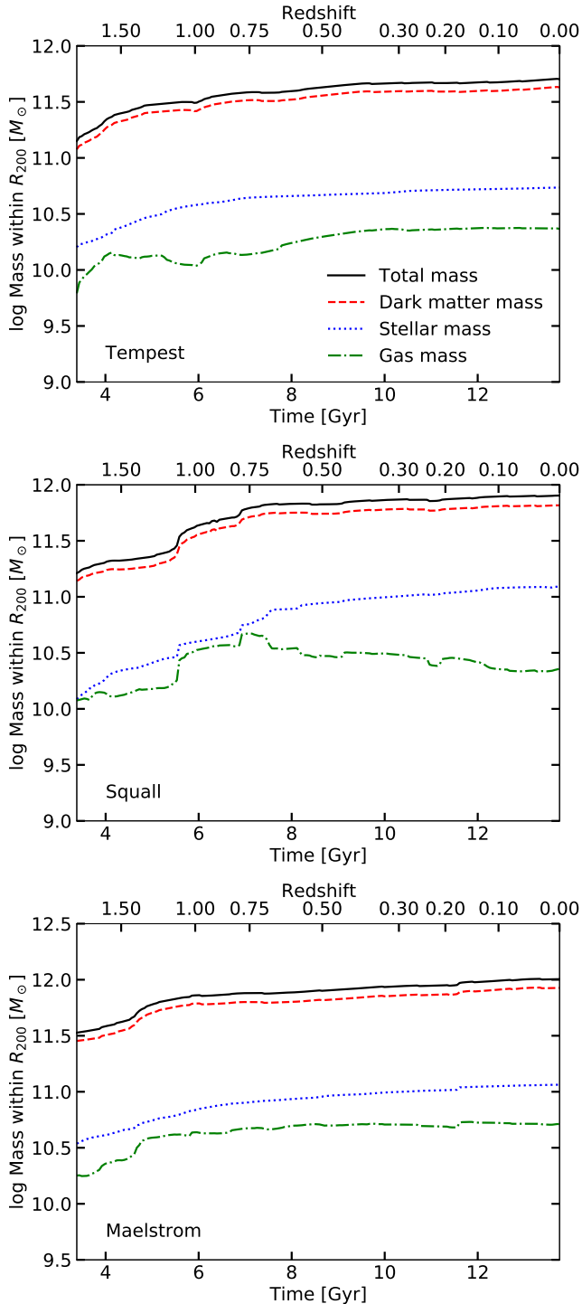
Figure 1. The total (black solid), dark matter (red dashed), stellar (blue dotted) and gaseous (green dash-dotted) masses within R_{200} for the three galaxies from the FOGGIE suite considered in this work, arranged from least massive to most massive at z = 0 top to bottom.
