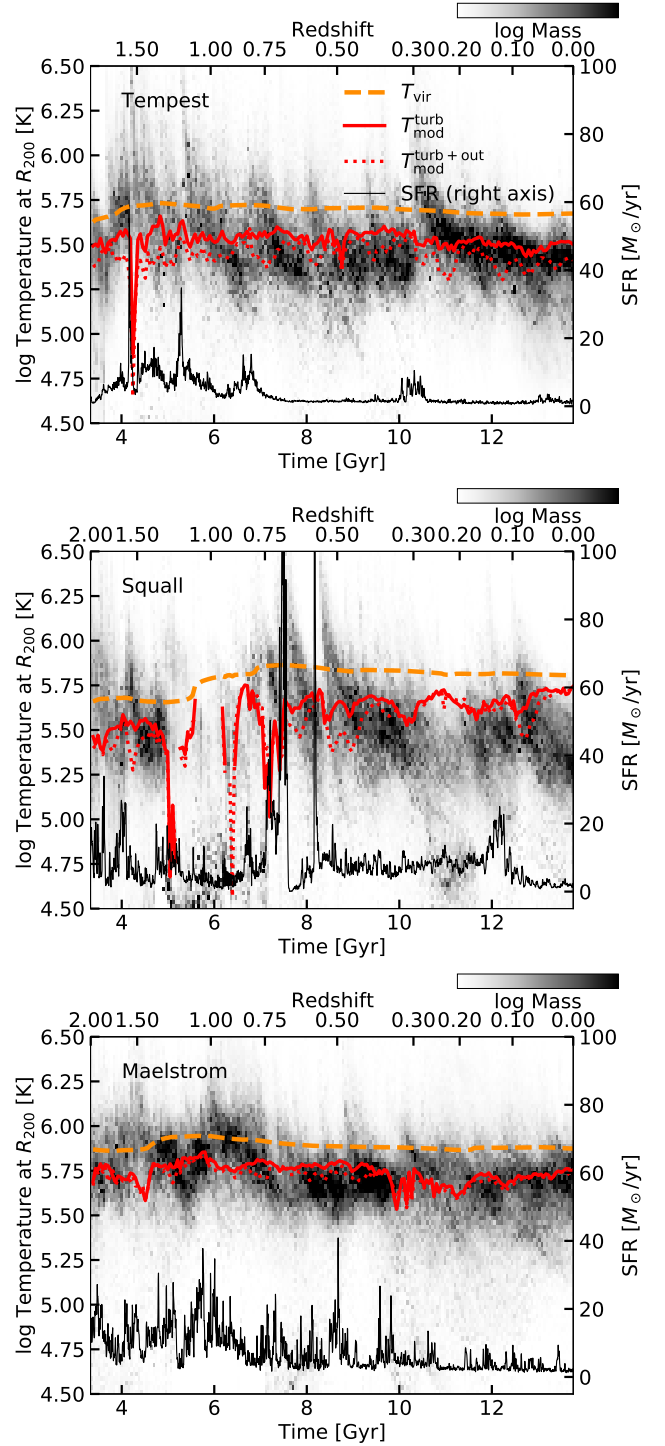
Figure 6. The temperature of gas with 0.99R_{200} < r < R_{200} is shown as a mass-weighted distribution as a function of cosmic time (bottom axis) and redshift (top axis), with dark colors indicating the peak of the mass-weighted temperature distribution. The orange dashed line shows the standard virial temperature (Equation 3) and red solid and red dashed lines show the modified virial temperature, calculated using the kinetic energy due to turbulence only (Equation 14) or both turbulence and outflows (Equation 15), respectively. The thin black line shows the star formation rate, with values on the right axis.
