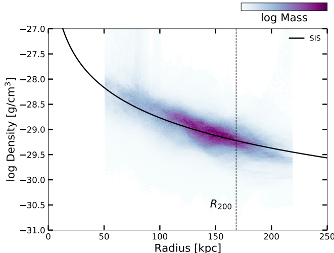
Figure 11. A mass-weighted histogram of warm halo gas density (filaments removed) as a function of radius. The black solid line shows a SIS density profile that is normalized to the gas density at R_{200} . The SIS profile describes the gas profile reasonably well.
