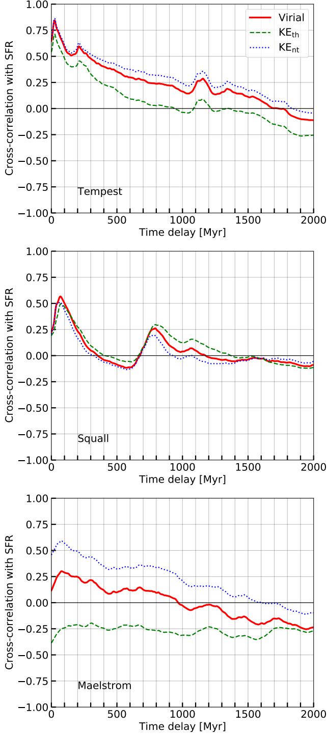
Figure 8. The cross-correlation between SFR and various energies of the gas near R_{200} as a function of time delay (Equation 16). The correlation is positive for \tau \lesssim 1 - 1.5 Gyr and peaks at \tau \sim 25 - 75 Myr, quantifying what is easy to see by eye in Figure 3, that the halo is driven out of virial equilibrium by strong bursts of feedback.
