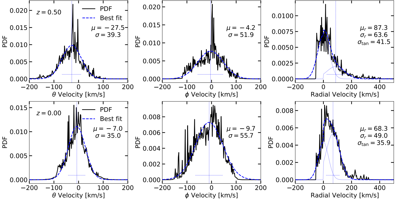
Figure 5. Mass-weighted distributions of velocities of gas within 0.99R_{200} < r < R_{200} are shown as the black solid lines, split into the three spherical directions: \theta (left), \phi (middle), and radial (right). The top row shows gas near R_{200} at z = 0.5 and the bottom row shows gas near R_{200} at z = 0 , both in the Tempest halo. The best-fit Gaussian model (to the two tangential velocity directions) and the best-fit double-Gaussian model (to the radial velocity direction) are shown as the blue dashed lines. For the double-Gaussian model, the two Gaussians that make it up are shown with thin blue dashed lines. Dotted vertical lines show the location of the best-fit mean of the Gaussian and dotted horizontal lines show \pm 1 best-fit standard deviation. The best-fit values are printed in each panel.
