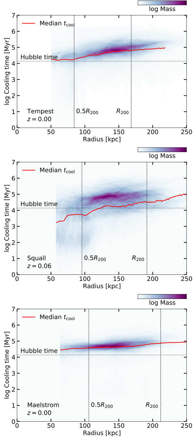
Figure 13. Histograms of gas cell cooling times (white-purple color shading) as functions of radius for each of Tempest, Squall, and Maelstrom at times when the halo gas is approximately virialized. The median cooling time is plotted as a red solid line. The bulk of the gas mass (dark purple colors) between 0.5R_{200} and R_{200} (dashed vertical lines) has cooling times a factor of \sim 2 - 8\times the Hubble time (horizontal dashed line), but there is a tail of cells with short cooling times that pull the median downward, especially in Squall, which is the furthest out of virial equilibrium.
