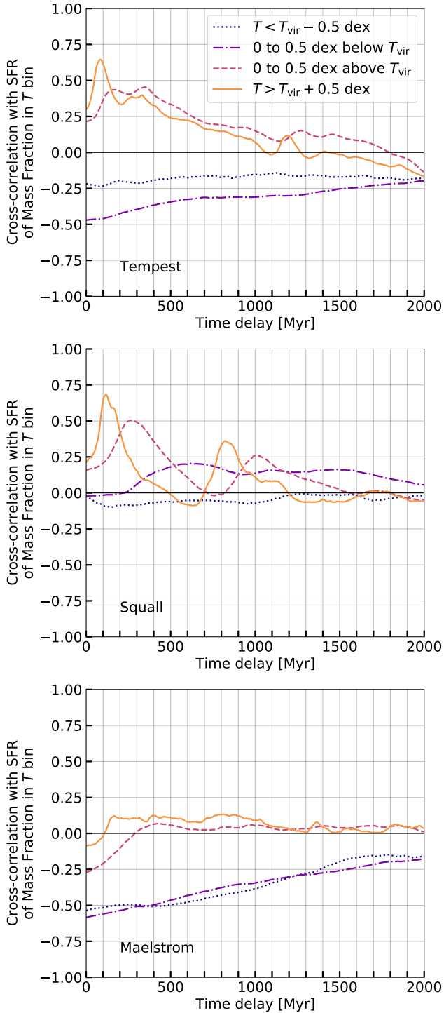
Figure 9. The cross-correlation between SFR and mass in different temperature bins relative to the standard T_{\text{vir}} as indicated in the figure, as a function of time delay \tau (Equation 16). The mass in the warmer temperature bins is positively correlated with SFR while the mass in the cooler bins is anticorrelated, quantifying what is easy to see by eye in Figure 6, that temperatures \gtrsim T_{\text{vir}} are only achievable following a burst of SFR and not when the halo is in relaxed virial equilibrium.
