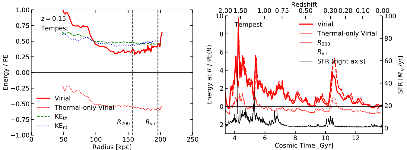
Figure 10. Left: The various energies of the gas in the Tempest halo at z = 0.15 , similar to Figure 4. Also marked as vertical dashed lines are two definitions of the halo radius, the R_{200} used throughout this paper and the virial radius R_{vir} . Right: The virial energies of the gas in the Tempest halo at R_{200} (solid lines) or R_{vir} (dashed lines), similar to Figure 3. There is little substantial difference in the virial energy (thick red line), between the definitions of halo radius.
