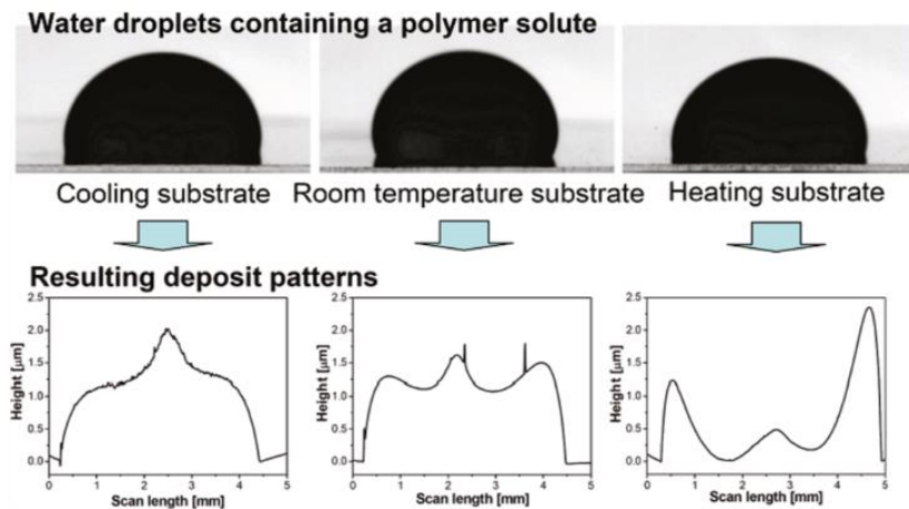
Fig. 3. Polymer solutions at various substrate temperatures and the height profile of the resulting deposit pattern. From (26).
