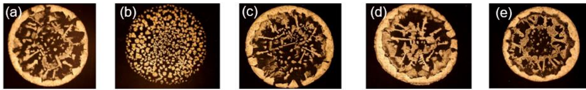
Fig. 19. Dried drop patterns from tequila adulterated with four different substances: (a) a control, (b) MEG (5 %v/v), (c) EtOH (10 %v/v), (d) Water (10 %v/v) and (e) MeOH (40 %v/v). From (87).
