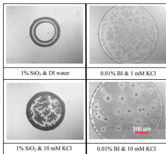
Fig. 5. Deposit pattern of nanoparticle suspensions with varying concentrations of salt (KCl). Modified from (29).
