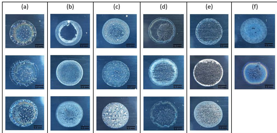
Fig. 23. Dried drop patterns from tap waters that underwent different treatments: (a) minimally
