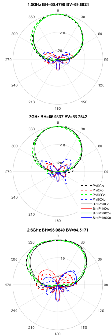
FIGURE 11. Simulated and measured radiation pattern.
