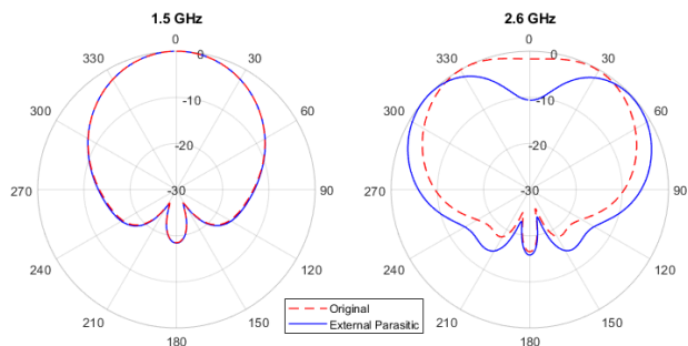
FIGURE 3. Radiation Pattern of External Parasitic Antenna present lobulation for highest part of frequency band (Discontinuous red line for original element, continuous blue line for external parasitic).
