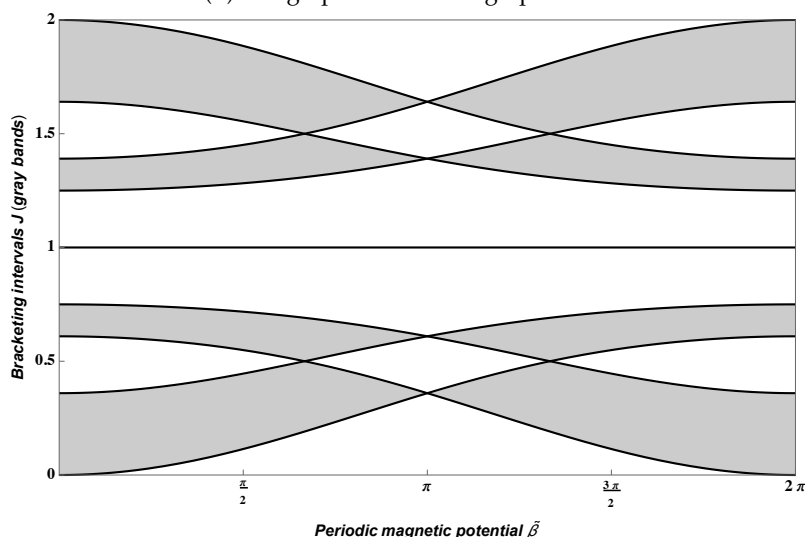
(c) Spectral bands and gaps as a function of the constant (periodic) magnetic potential \tilde{\beta} .
