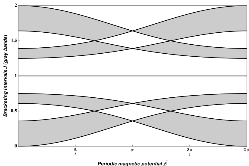
Figure 3. The horizontal axis represents the values of the magnetic potential \tilde{\beta} \in [0, 2\pi) acting on the polyacetylene polymer with standard weights. For any fixed \tilde{\beta} we obtain the intervals J given by the bracketing technique as we did in the case \tilde{\beta} = \pi/2 in Figure 2 (and also using the symmetry given by the bipartiteness). In the vertical axis, we represent the spectral bands and gaps for each constant value \tilde{\beta} .
