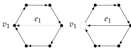
(b) The graph \mathbf{G}^- and the graph \mathbf{G}^+ .
