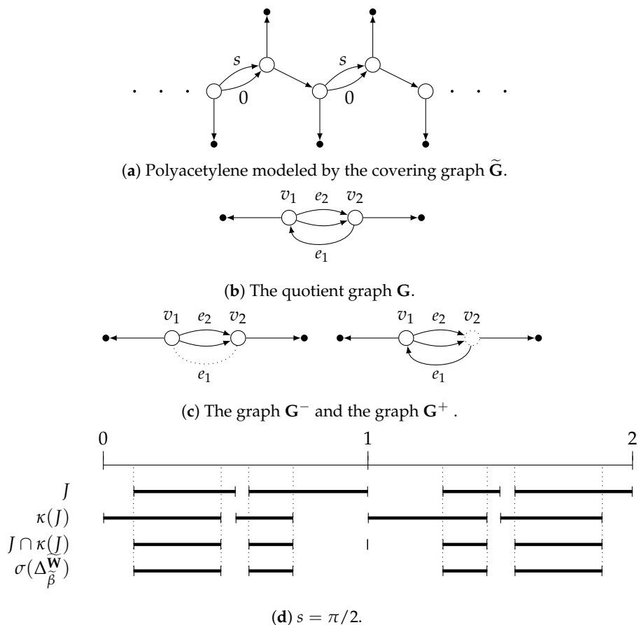
Figure 2. Spectral gaps of the polyacetylene graph for a constant magnetic potential \beta = s . Here, J is the spectral localization for the pair \mathbf{G} - \{e_1\} and \mathbf{G} - \{v_1\} . Bipartiteness gives a finer localization J \cap \kappa(J) . In this case, we obtain the spectrum almost exactly, except for the spectral value 1.
