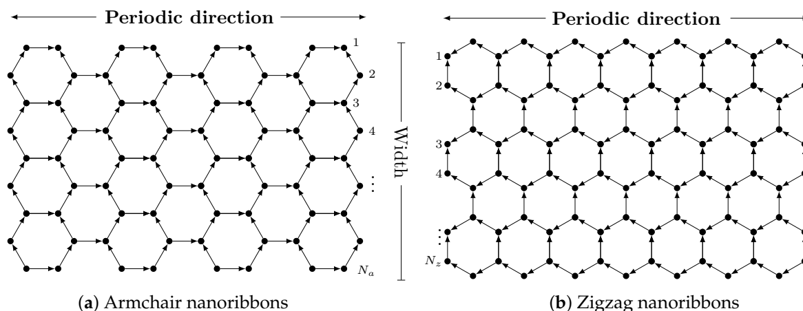
Figure 5. Two structures of the graphene nanoribbons: armchair and zigzag. These structures are covering graphs only in one direction.
