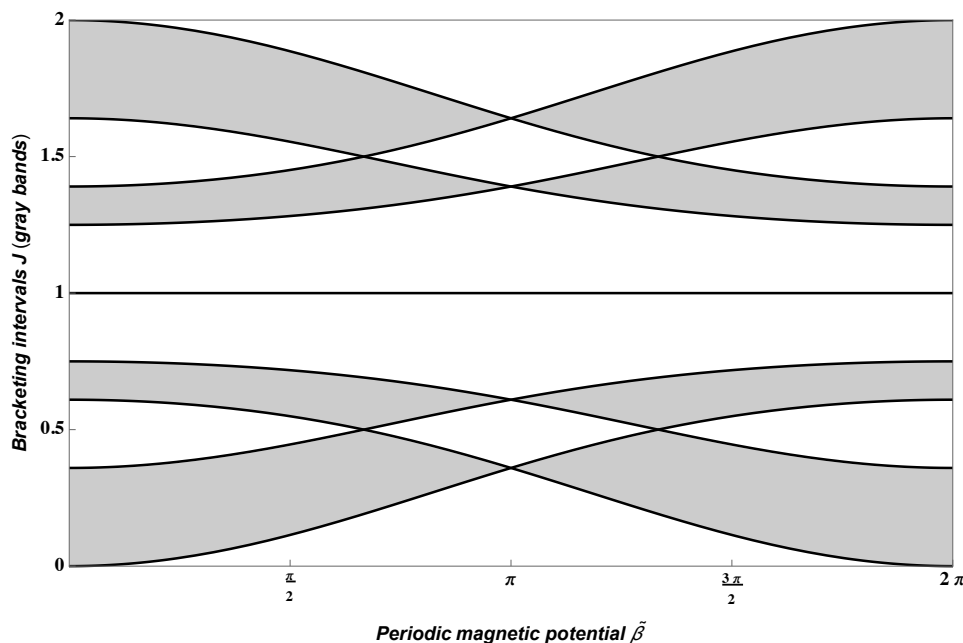
Figure 1. The structure of the bracketing intervals J is represented with gray bands and the spectral gaps with white bands. Both bands depend on the constant (periodic) magnetic potential \tilde{\beta} acting on 3- a GNR.
