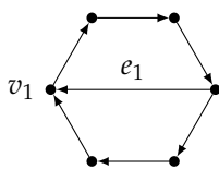
(a) The quotient graph \mathbf{G} of 3-aGRN.
