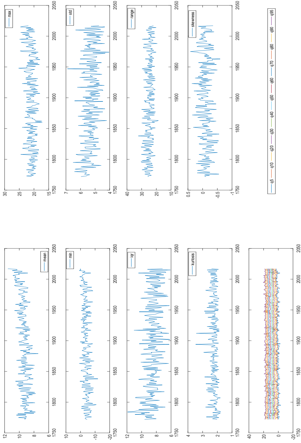
Figure 3 Annual temporal distributional characteristics of Central England temperature (degrees Celsius) calculated with daily data
