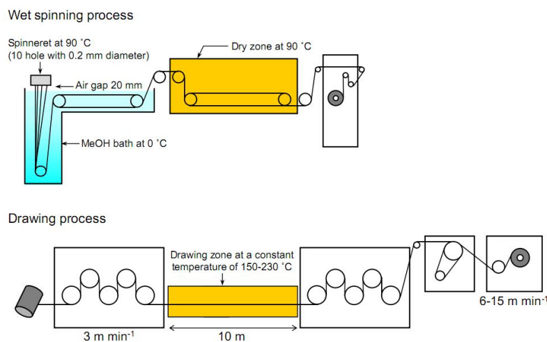
Figure 11. Scheme showing all stages during dry-wet spinning process (reprinted from Polymer , 2013, 54, 935–914, Endo, R.; Saito, T.; Isogai, A. TEMPO-oxidized cellulose nanofibril/poly(vinyl alcohol) composite drawn fibers, with permission from Elsevier).
