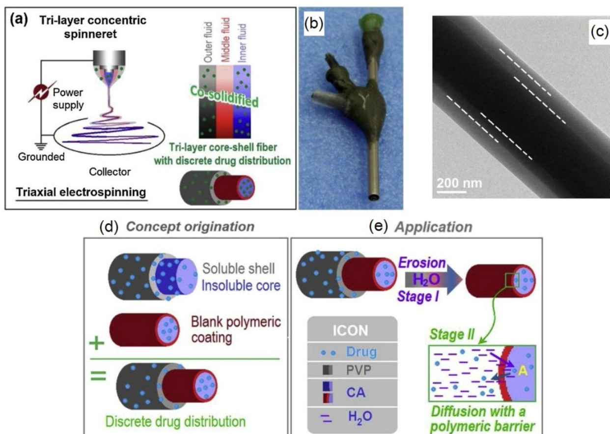
Figure 13. A scheme of triaxial electrospinning (a); triaxial spinneret (b); tricompnent fiber (c); scheme of the concept for triaxial spinning (d); application of tricompnent fiber for sustainable drug release (e) (reprinted and adapted from Carbohydrate Polymers , 2020, 243, 116477, Yang, Y.; Chang, S.; Bai, Y.; Du, Y.; Yu, D.G. Electrospun triaxial nanofibers with middle blank cellulose acetate layers for accurate dual-stage drug release, with permission from Elsevier).
