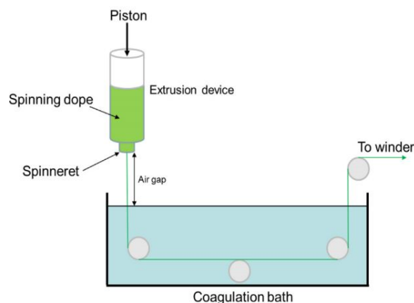
Figure 10. General scheme of dry-jet wet spinning using air gap between spinneret and coagulation bath (reprinted from International Journal of Biological Micromolecules , 2016, 92, 1197–1204, Boy, R.; Narayanan, G.; Chung, C.C.; Kotek, R. Novel cellulose-collagen blend biofibers prepared from an amine/salt solvent system, with permission from Elsevier).
