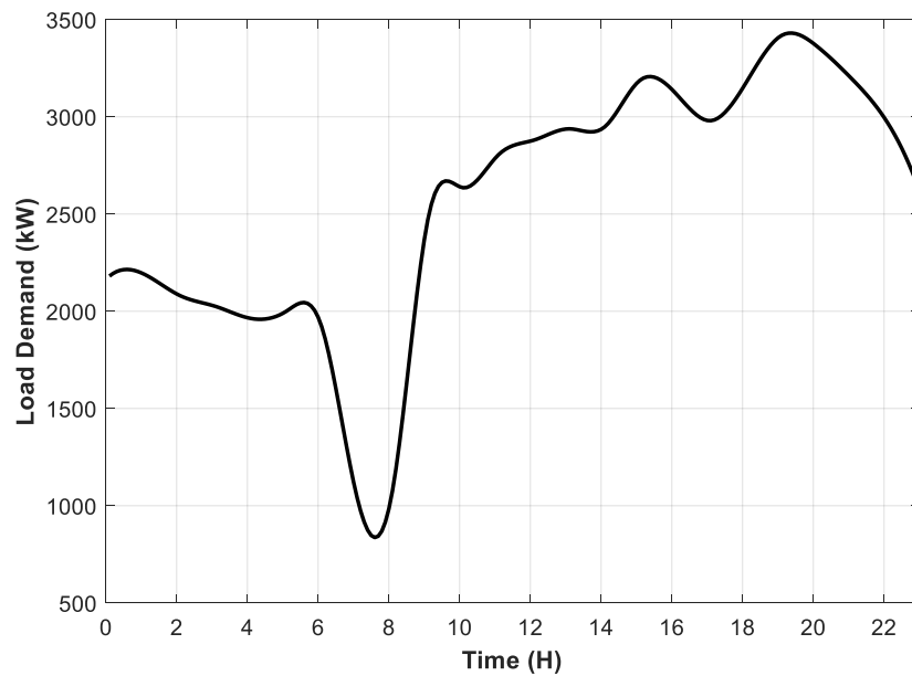
Figure 2. Load demand.
