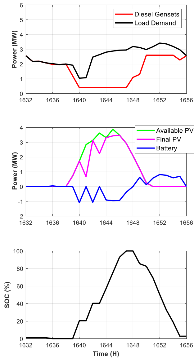
Figure 6. Microgrid operation for one day in summer using the optimal EMS Strategy.
