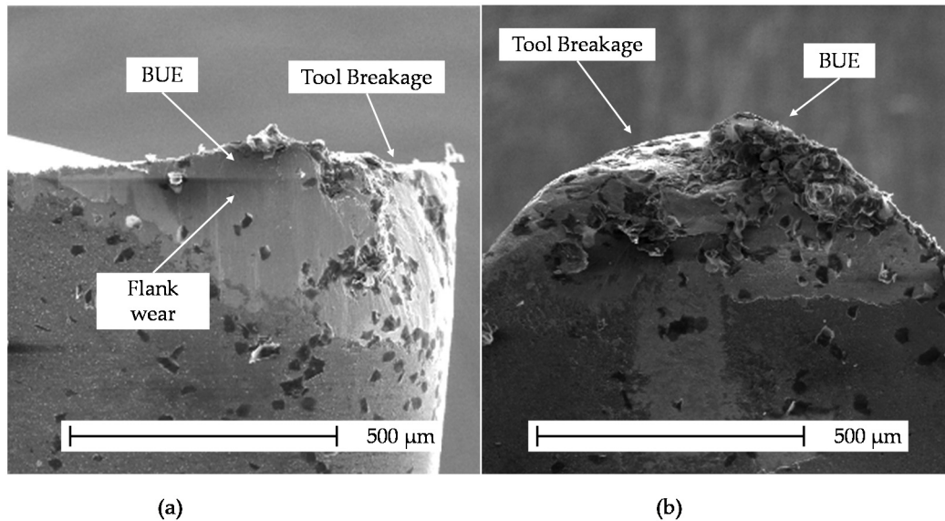
Figure 8. SEM images of the tool at the end of the tool life corresponding to Haynes 282 under conventional pressure with cutting speed 50 m/min and feed 0.15 mm/rev: (a) relief surface view, (b) rake surface view [36].
