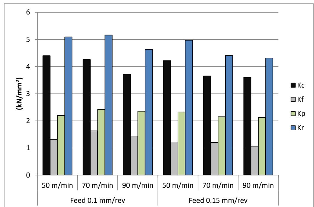
Figure 3. Initial k_c , k_f , and k_p forces for turning tests on Haynes 282 with high pressure cooling.
