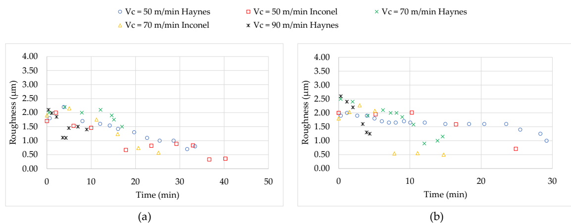
Figure 11. Machined surface roughness for Haynes [36] and Inconel [38] under conventional cooling pressure: (a) feed = 0.1 mm/rev, (b) feed = 0.15 mm/rev.
