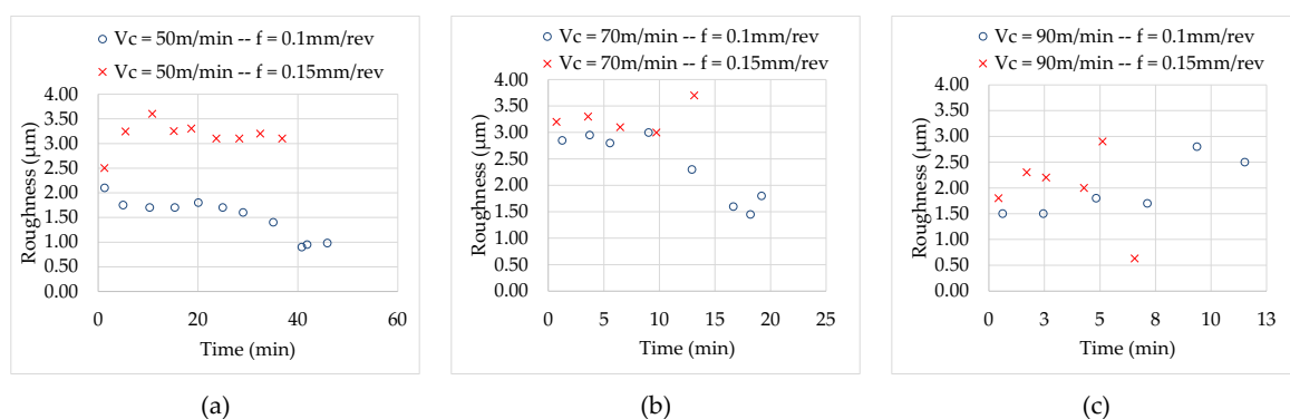
Figure 10. Machined surface roughness for Haynes 282 turning tests with high pressure cooling: (a) 50 m/min; (b) 70 m/min and (c) 90 m/min.
