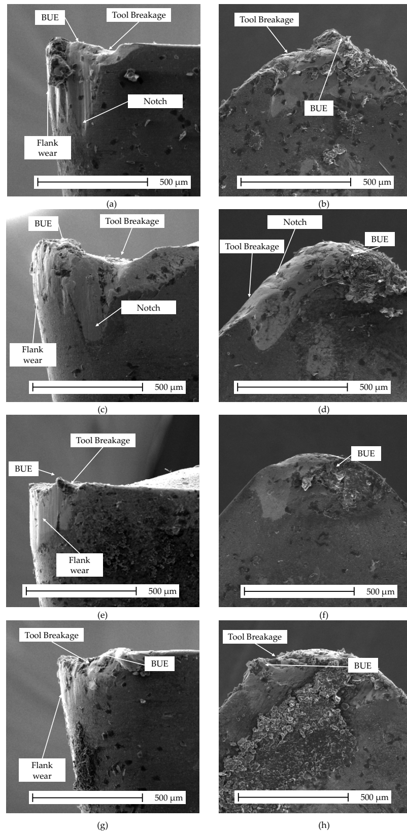
Figure 7. SEM images at the end of the tool life for different cutting conditions in Haynes 282 turning tests with high pressure cooling. For 50 m/min and 0.1 mm/rev: (a) relief surface and (b) rake surface view. For 50 m/min and 0.15 mm/rev: (c) relief surface and (d) rake surface view. For 90 m/min and 0.1 mm/rev: (e) relief surface and (f) rake surface view. For 90 m/min and 0.15 mm/rev: (g) relief surface and (h) rake surface view.
