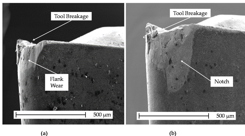
Figure 9. SEM images of the tool at the end of the tool life corresponding to Inconel 718 under conventional pressure with: (a) cutting speed 50 m/min and feed 0.1 mm/rev, (b) cutting speed 70 m/min and feed 0.15 mm/rev [38].
