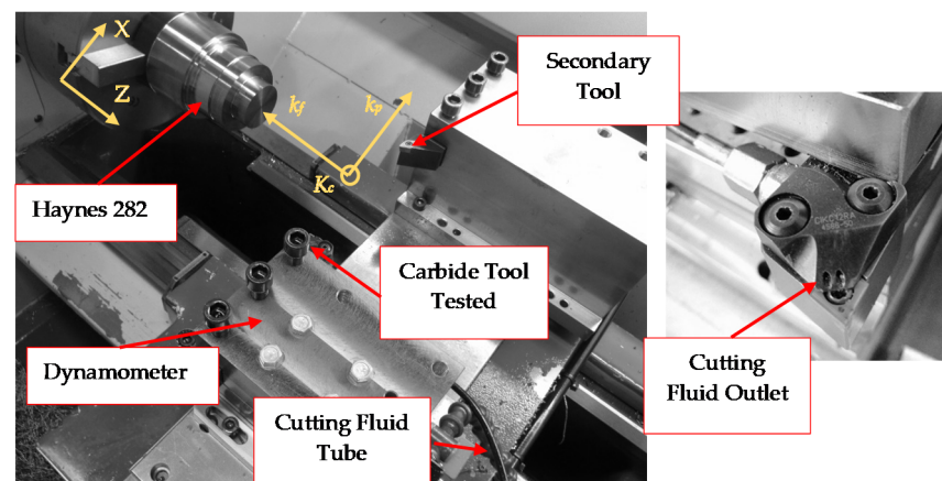
Figure 2. Experimental setup.
