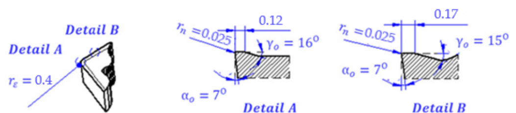
Figure 1. Coated carbide tool configuration. Reprinted with permission from ref. [18]. Copyright 2021 Elsevier. Measurements in mm.
