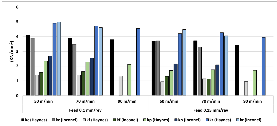
Figure 4. Initial specific cutting forces for both Haynes [36] and Inconel [38] under conventional pressure.
