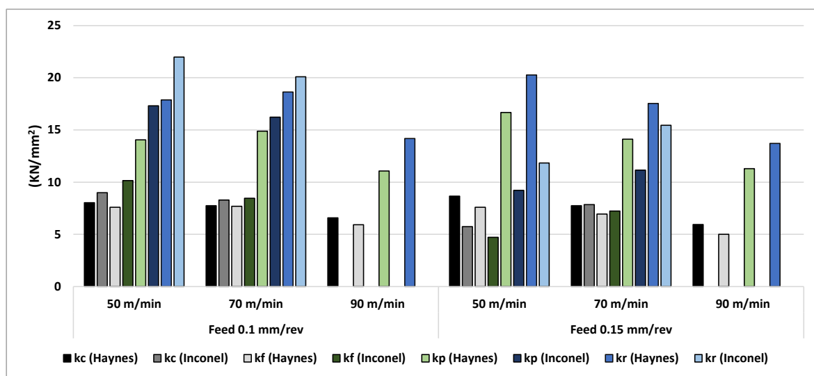
Figure 6. Specific cutting forces for both Haynes [36] and Inconel [38] under conventional pressure with worn tool.
