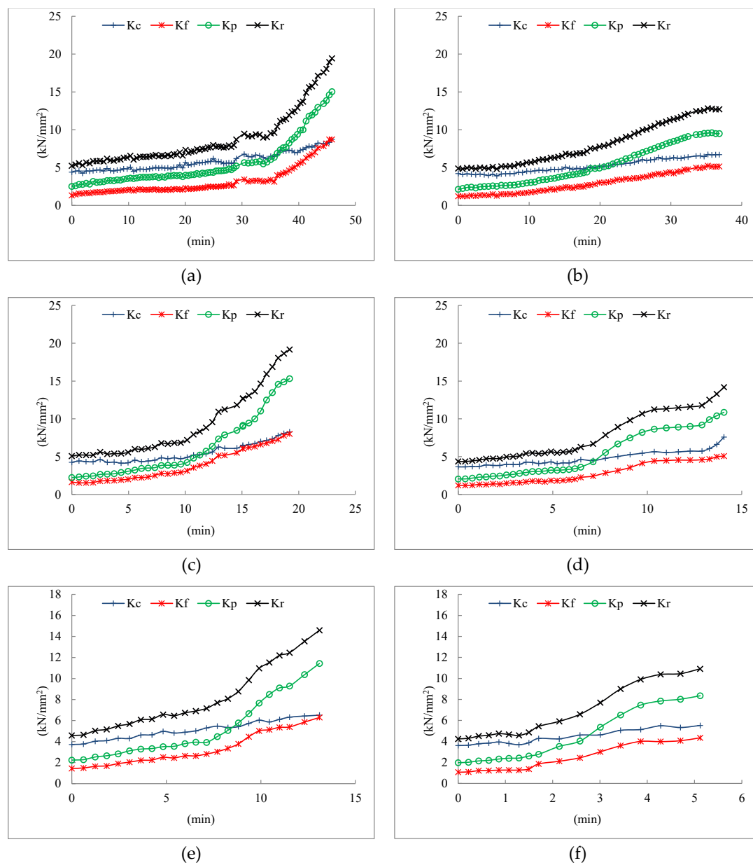
Figure 5. Cutting forces progression for Haynes 282 turning tests with high pressure cooling. (a) V_c = 50 m/min and f = 0.1 mm/rev; (b) V_c = 50 m/min and f = 0.15 mm/rev; (c) V_c = 70 m/min and f = 0.1 mm/rev; (d) V_c = 70 m/min and f = 0.15 mm/rev; (e) V_c = 90 m/min and f = 0.1 mm/rev; (f) V_c = 90 m/min and f = 0.15 mm/rev.
