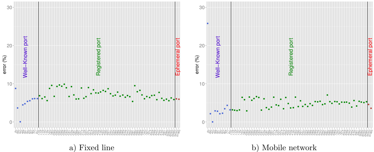
Figure 2: Error rate vs. port number.
