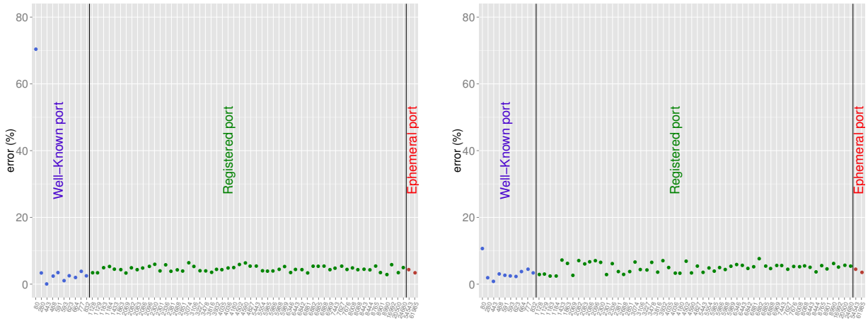
a) Mobile proxy b) Mobile non-proxy Figure 3: Error rate vs. port number.
