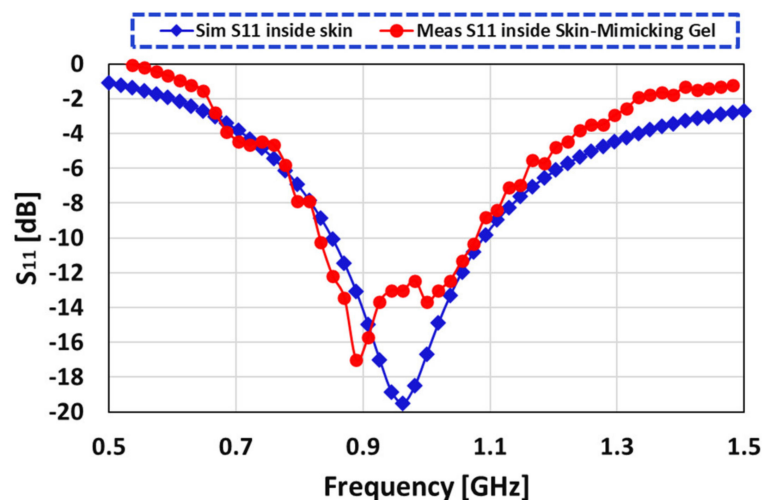
Figure 9. Contrast between the simulation and measurement results of S_{11} inside skin-gel.
