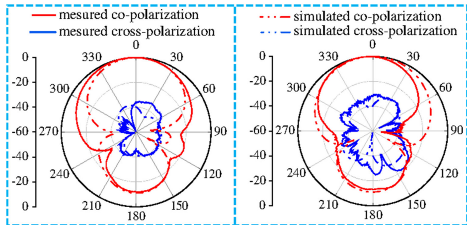
Figure 10. Simulation and measurement far field results at 915 MHz inside the skin-gel.
