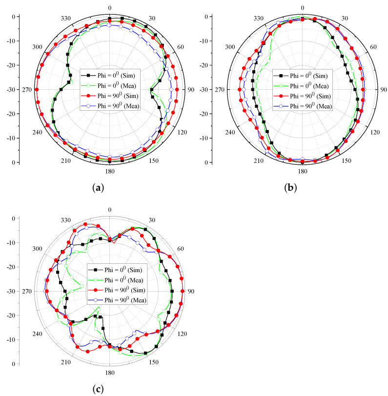
Figure 13. Radiation characteristics of the proposed UWB MIMO for port-4. (a) 3 GHz. (b) 6 GHz. (c) 9 GHz.
