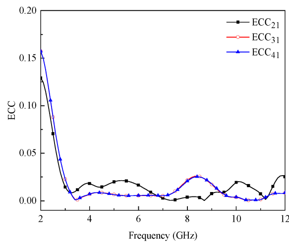
Figure 14. ECC of the proposed UWB MIMO antenna.
