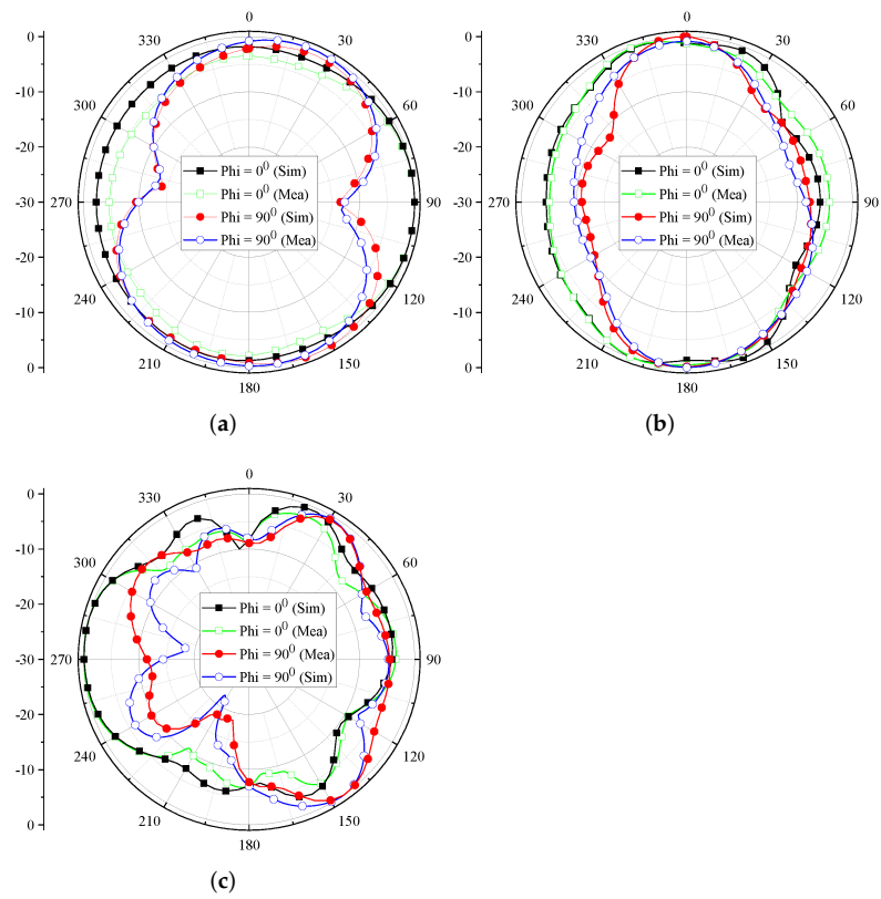
Figure 10. Radiation characteristics of the proposed UWB MIMO for port-1. (a) 3 GHz. (b) 6 GHz. (c) 9 GHz.
