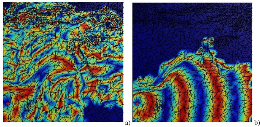
Fig. 29 Difference between the wave expansion D matrices when the robot has and hasn't data of the points lower than its altitude.
