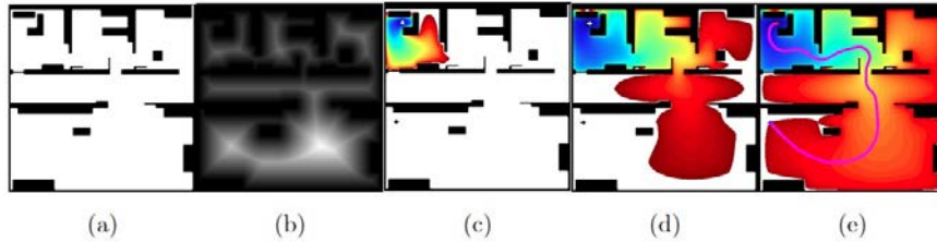
Fig. 5 Example of environment a), first potential b) and tree moments of the wave expansion c) d) and e). In the last is shown the corresponding path.
