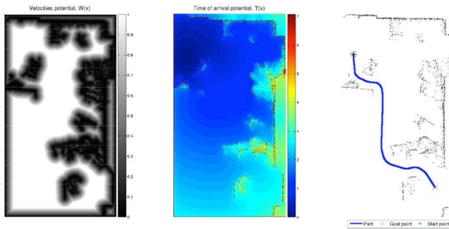
Fig. 8 First potential, second potential and the path corresponding to a medium level of saturation.
