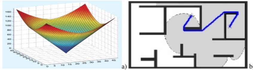
Fig. 2 Lyapunov surface when the propagation wave starts in a point and the refraction index is constant (a) and Fast Marching Path when the refraction index is constant (b)
