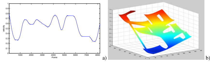
Fig. 4 a) Relative velocity profile of the path obtained in the previous figure, where 1 is the maximum velocity and b) its Lyapunov surface.
