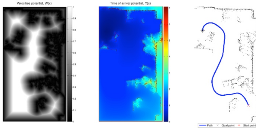
Fig. 9 First potential, second potential and the path corresponding to a low level of saturation.
