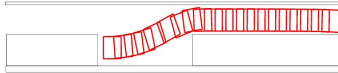
Fig. 20 Parking maneuver using FM 2 -NH.
