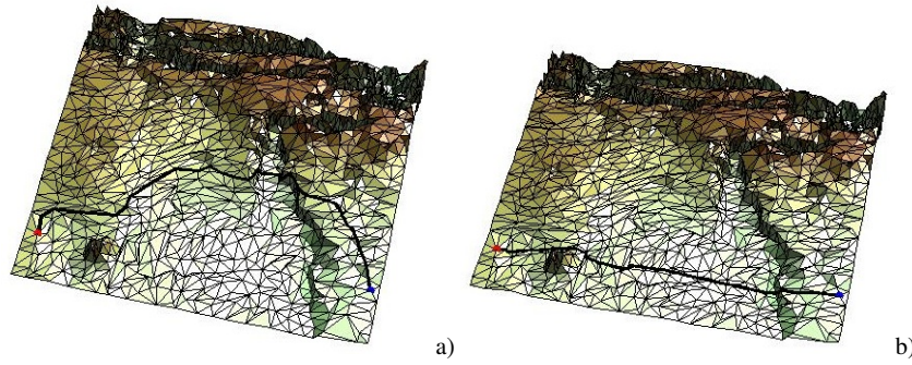
Fig. 27 Difference between the robot trajectories a) without and b) with uncertain data of the points lower than its altitude.
