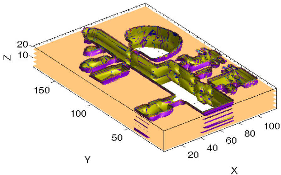
Fig. 19 Three dimensional C-space of the car-like robot, where the third dimension is the orientation. These orientations are repeated above and under the principal interval in order to permit manoeuvres
