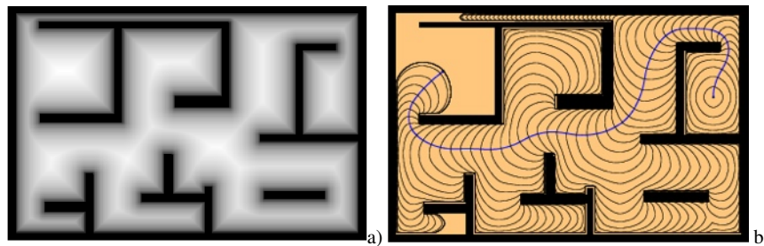
Fig. 3 a) Repulsive field by propagating a wave from the obstacles and walls (first potential) and b) the corresponding wave fronts and its Fast Marching Path when the refraction index is given by a)
