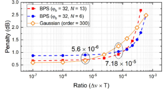
Fig. 10. Simulation results comparing the blind and pilot tone-assisted PNC techniques. The results obtained at the (\Delta\nu \times T) ratios used in the transmission experiments are marked with circles.
