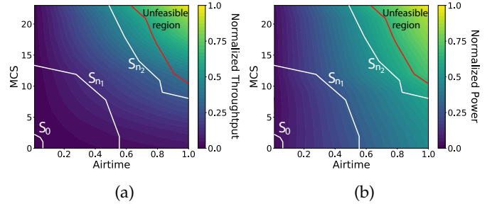
Fig. 6: Example of safe set expansion in the uplink throughput and power domains as a function of two decision variables: uplink MCS and uplink airtime. As SBP-vRAN explores, the initial safe set S_0 is expanded until it reaches the boundary of the unfeasible region, where the optimum is located.
