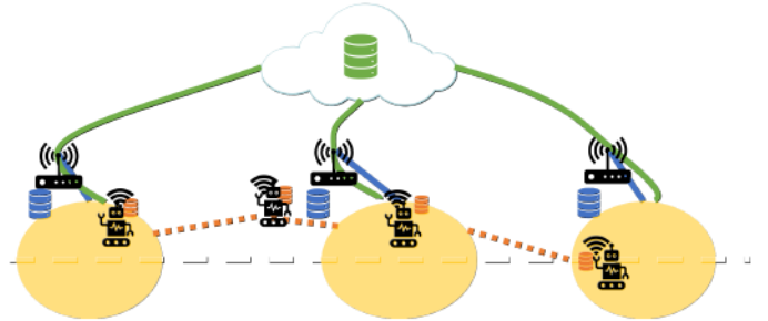
Fig. 1. As per geographical availability requirements, a mobile robot, smart factory service must be provided within the yellow areas, with high reliability and low latency. This can be obtained by deploying: (a) service instances at the robots (fog resources), at lower cost but also lower reliability, hence, needing redundancy to meet reliability constraints (orange option); (b) three instances at the points of attachment (PoA), e.g., access points (APs), covering the target areas (edge resources, blue option); (c) deploying only one instance in the cloud, but with larger delay (green option).
