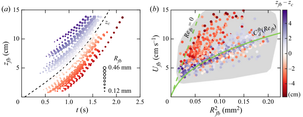
Figure 6. (a) Vertical trajectories of ‘free’ bubbles sufficiently separated from the thermal core (thermal x ). The dashed black curve outlines the vertical trajectory of the thermal centroid (third-degree polynomial fit, extrapolated for z_c > 12 cm). Data points are size-coded by the bubble radius R_{fb} and are colour-coded based on the instantaneous vertical distance from the bubble to the centroid height: z_{fb} - z_c ; see colourbar in (b). (b) Absolute bubble speed as a function of R_{fb}^2 for the bubbles shown in (a). The solid line plots the terminal velocity in (3.2), i.e. for a massless solid sphere following the standard drag curve; the dashed line plots Stokes’ terminal velocity (3.1). The grey shaded area delimits the experimental space for all the free bubbles analysed from all 19 thermals.
