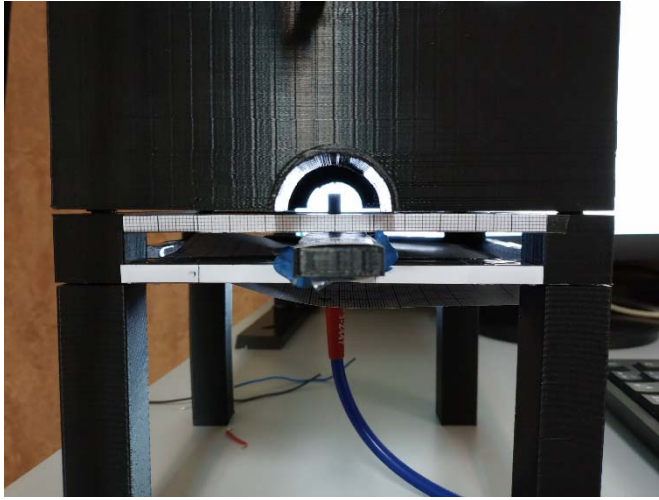
Fig. 8. (a) Calibration and measurement system are used to extract the experimental data. (b) Then, we compare these data with the simulations obtaining a good match.
