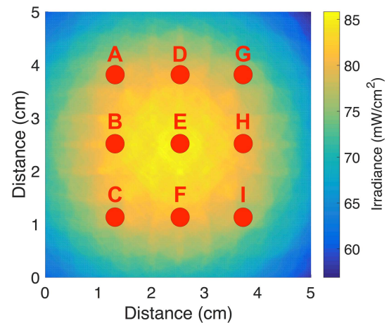
Fig. 2. Simulated irradiance spatial distribution with nine calibration points.
