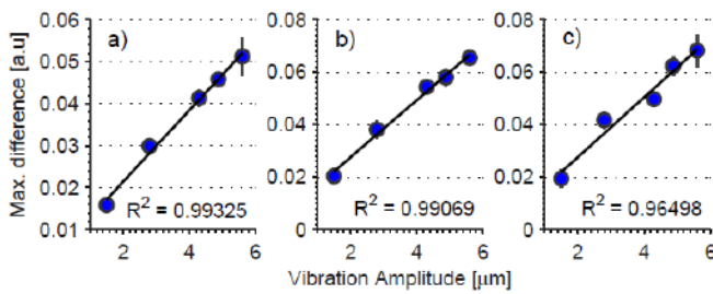
Fig. 9. Maximum variation of GR = Corr(G) \times Corr(R) when the vibration source is placed at points: a) P 1 , b) P 5 and c) P 9 .
