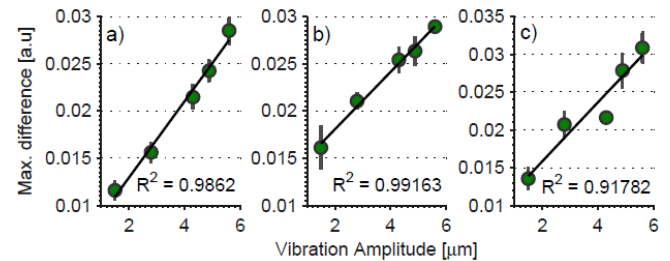
Fig. 8. Maximum variation of Corr(G) in the time domain when the vibration source is placed at points: a) P_1 , b) P_5 and c) P_9 .
