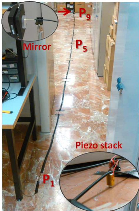
Fig. 3. Experimental set-up of the remote system for micro-vibrations detection. The sensing fiber is a standard SI-POF fiber of 11m-long with a 2.2 mm jacket directly attached to the floor. A piezoelectric stack is used to emulate periodic perturbations with amplitudes ranging from 1 to 6 \mu\text{m} at points P1, P5 and P9, respectively
