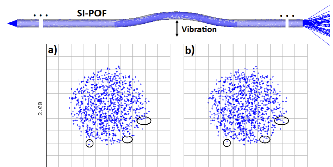
Fig. 2. Simulations of the speckle pattern variation in a SI-POF lead of 2 m, \lambda = 520\text{ nm} . The vibration's amplitude in b) is 1\ \mu\text{m} greater than in a).
