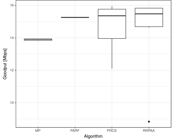
Figure 10: Goodput achieved per simulated algorithm.
