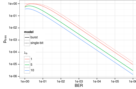
Figure 5: Frame loss probability given a BER level.
