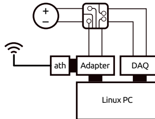
Figure 2: Measurement setup for energy performance characterisation.
