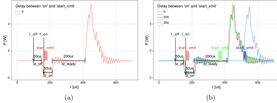
Figure 3: Atheros AR9280 timing characterisation.
