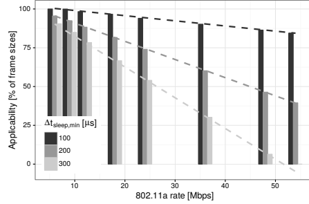
Figure 11: Algorithm applicability for common transmissions ( \leq 1500 bytes + ACK) in 802.11a DCF mode.
