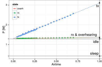
Figure A.12: Atheros AR9280 power consumption in 11a mode.
