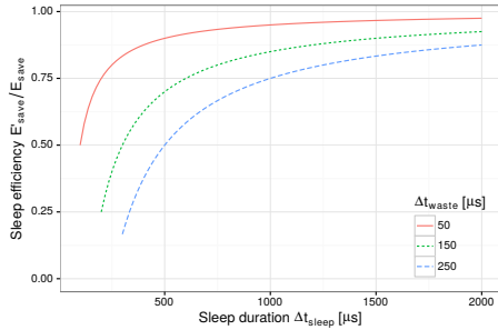
Figure 10: Sleep efficiency behaviour as \Delta t_{\text{waste}} decreases.
