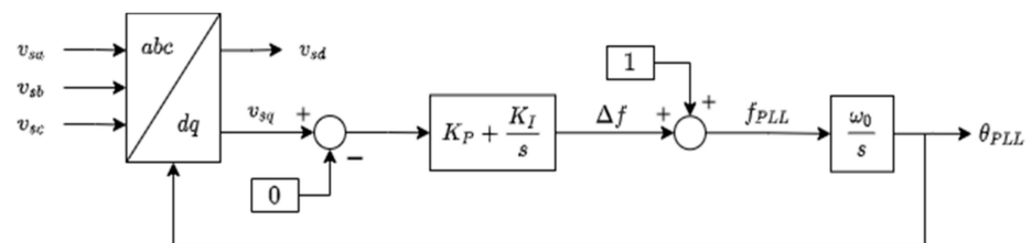
Figure 2. Phase Locked Loop scheme.
