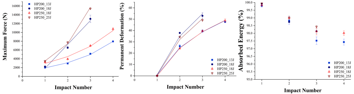
Fig. A1. Maximum force, permanent deformation and percentage absorbed energy trends with increasing number of impacts of HP200 tested at 13 J and 18 J and of HP250 tested at 18 J and 25 J
