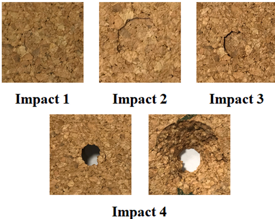
Fig. 11. Damage progression of NL25 sample impacted at 2.5 J.
